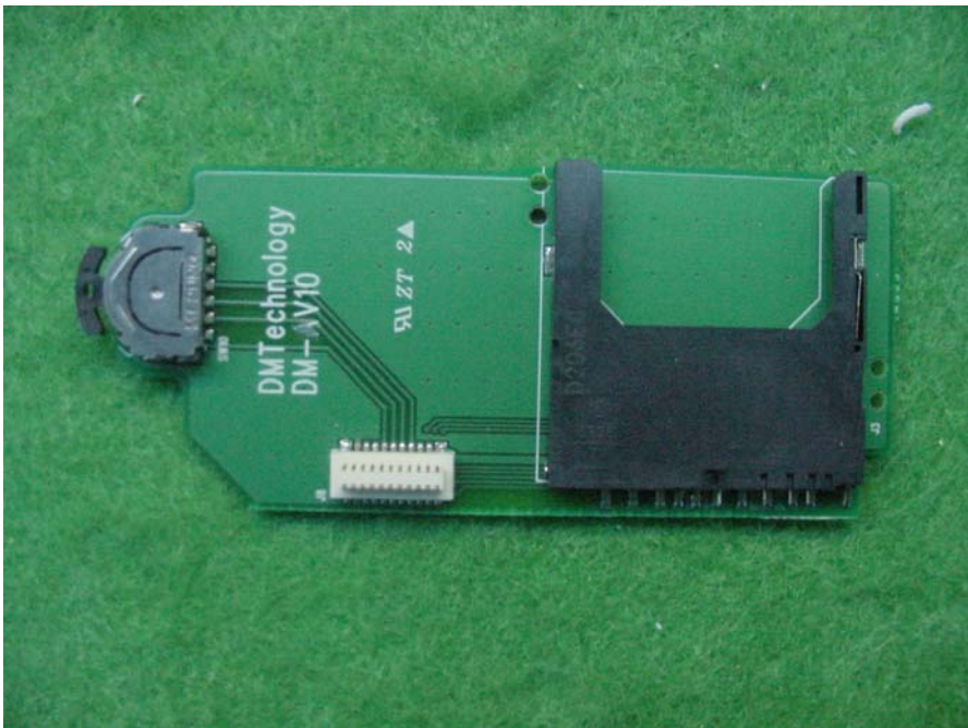
< Front Photo of Memory Slot Board >
