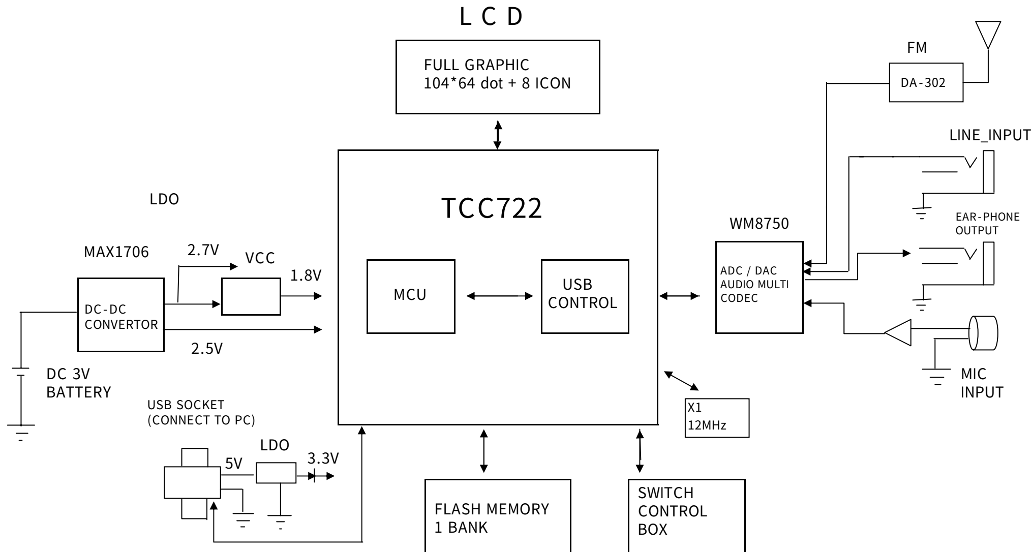
DM-FA60 BLOCK DIAGRAM
