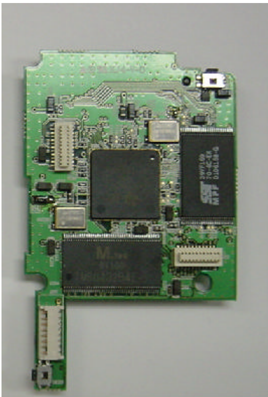
<MAIN BOARD>
