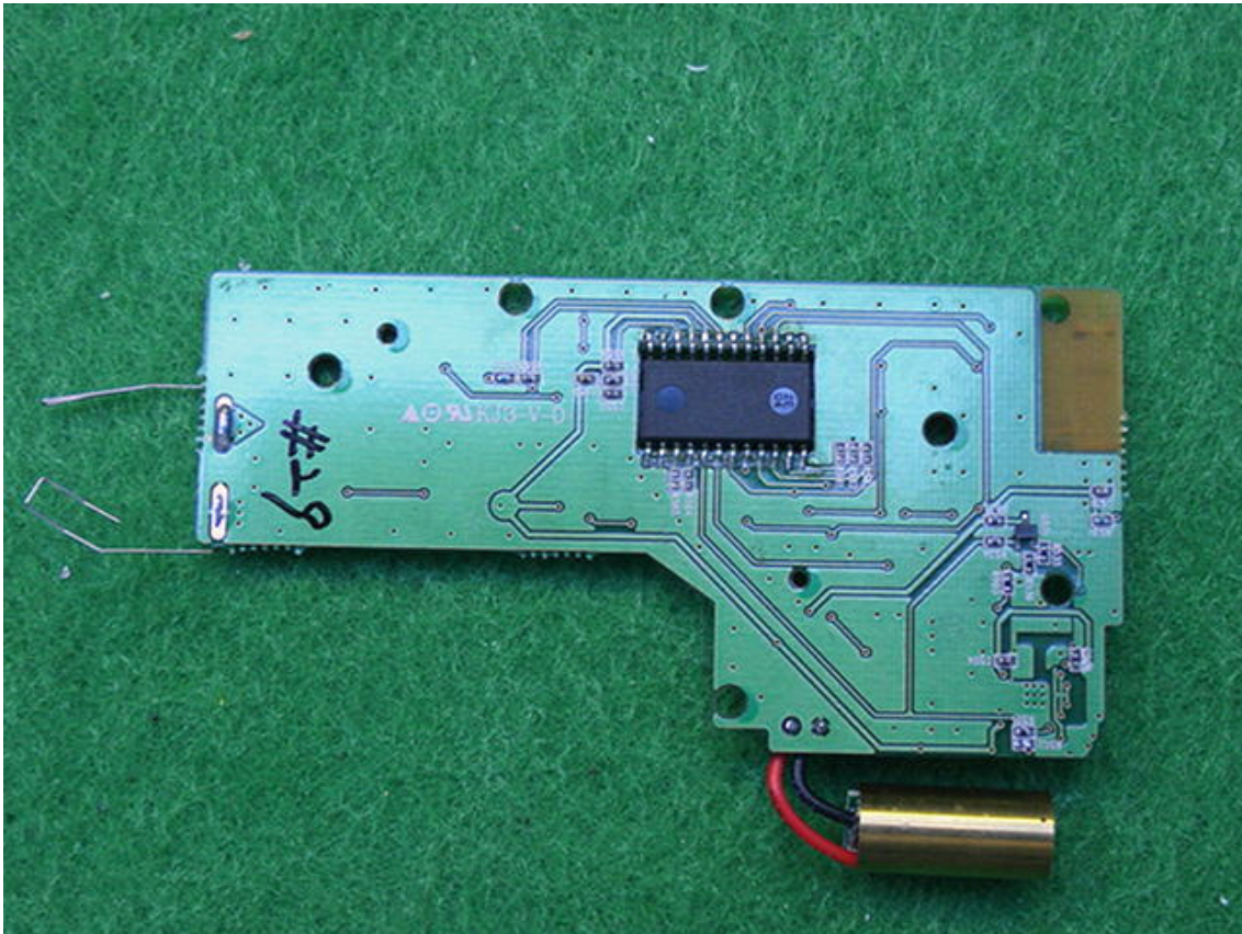
<REMOTE CONTROLLER>
