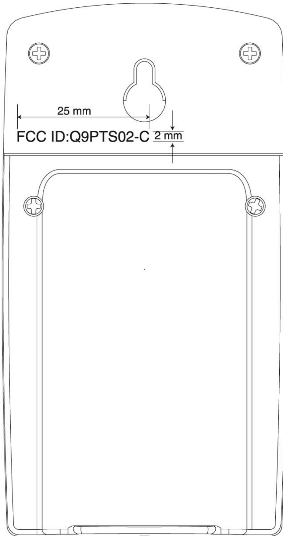
NILBRAND TS02 REAR CASE SILKSCREEN COLOR: BLACK FOR WHITE CASE BY WING TSUI 10/07/03
