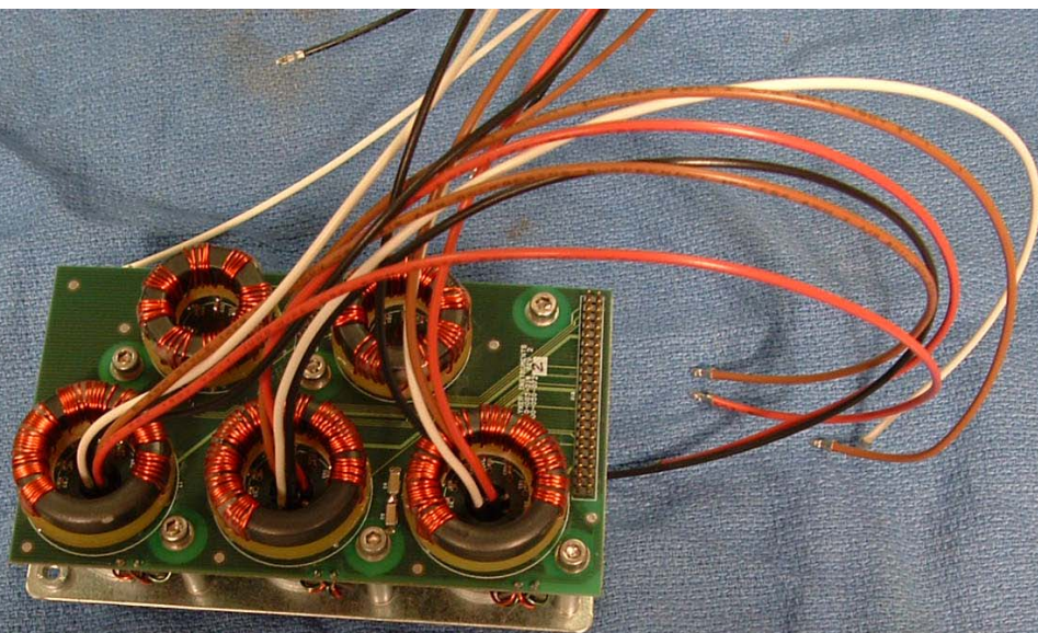
Connector Harness PCB
