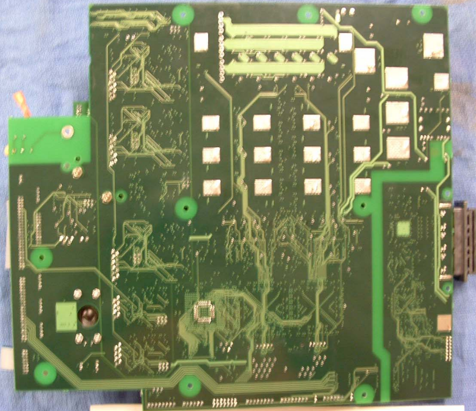
Main PCB
