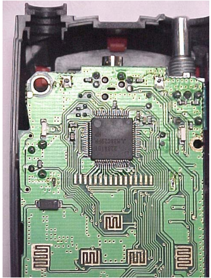
Mainboard with LCD Removed
