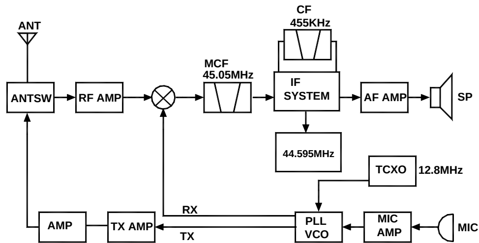
Figure 1 frequency configuration
