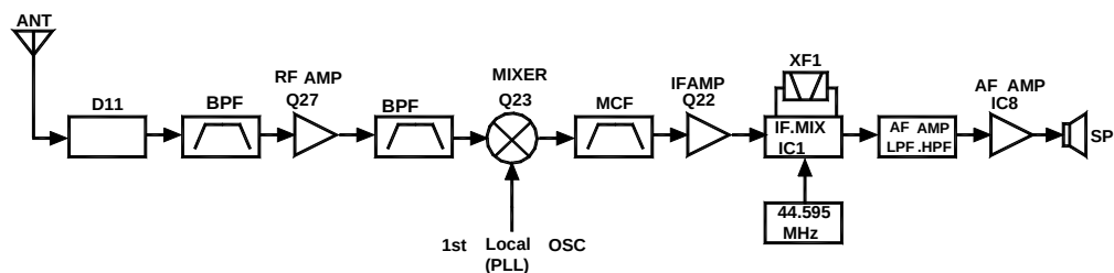
Figure 2 receiver section configuration
