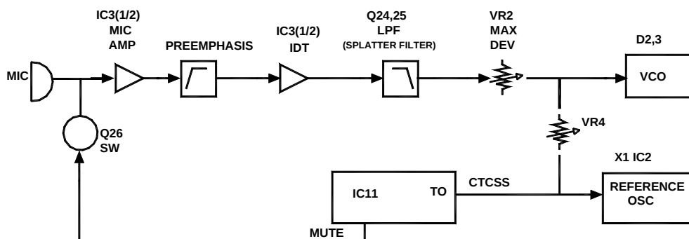
Figure 6 transmit CTCSS
