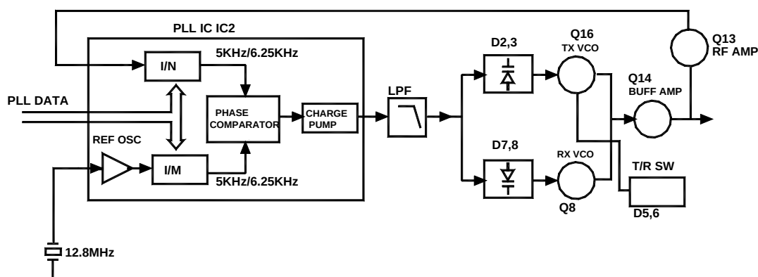
Figure 4 PLL circuit
