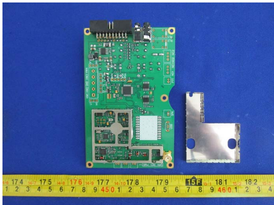
EUT – Bottom Uncover View
