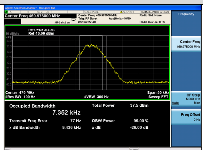
12.5kHz, 4FSK Modulation:469.975MHz
