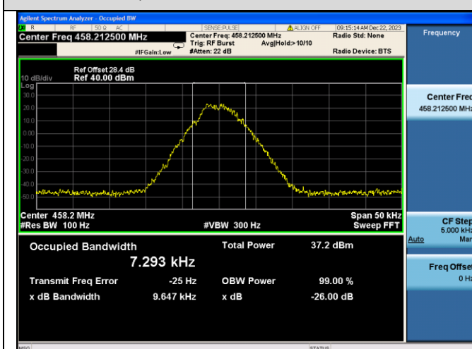
12.5kHz, 4FSK Modulation:458.2125MHz
