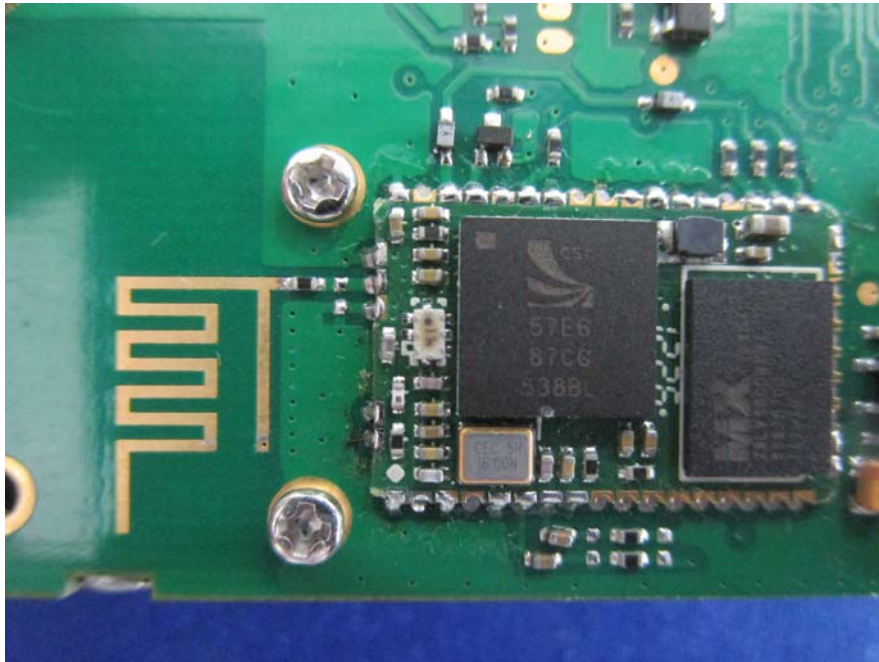
EUT –BT Chip & Antenna View
