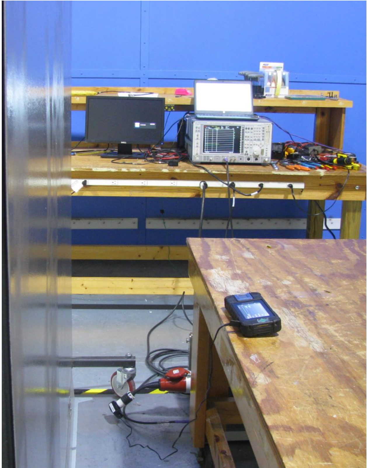
Conducted Emissions
