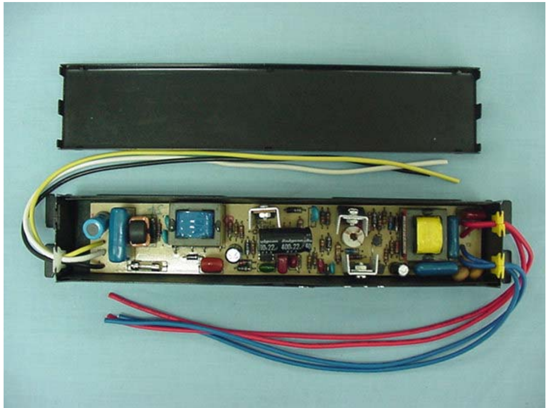
FIGURE 1 ELECTRONIC BALLAST (M/N: FBT T5 28) COVER REMOVED
