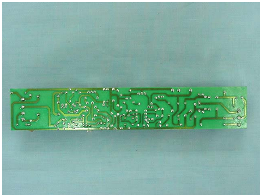
FIGURE 3 ELECTRONIC BALLAST (M/N: FBT T5 28) MAIN BOARD (SOLDERED SIDE)
