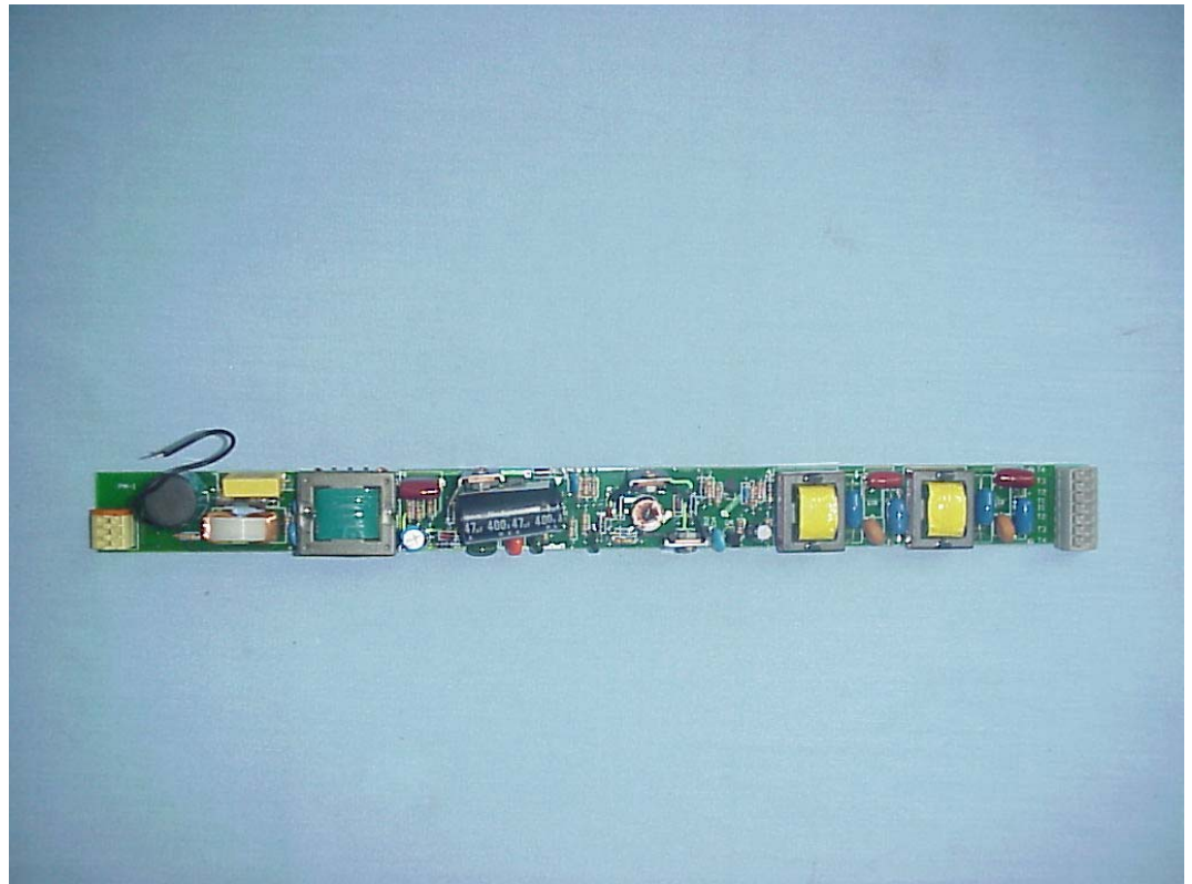
FIGURE 3 BALLAST (M/N: FBT T5 28x2) MAIN BOARD (COMPONENT SIDE)
