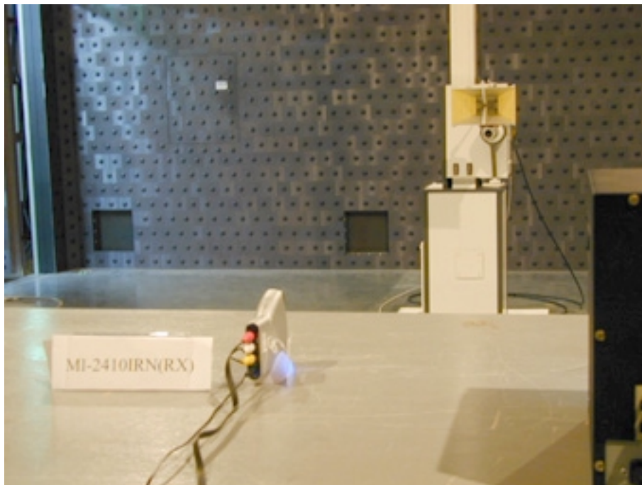
Photo 4: Spurious Set-up
