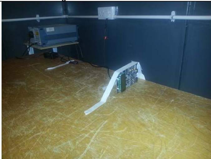
Fig 5 Conducted Emissions -
