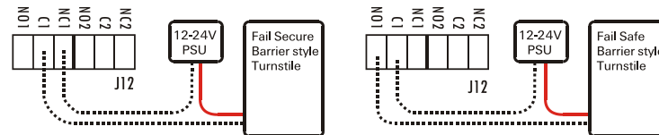
Sample wiring for a uni-directional turnstile barrier with external PSU.
