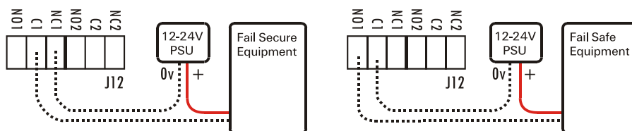
An example of S610S PCB connections used for Equipment Mode.
