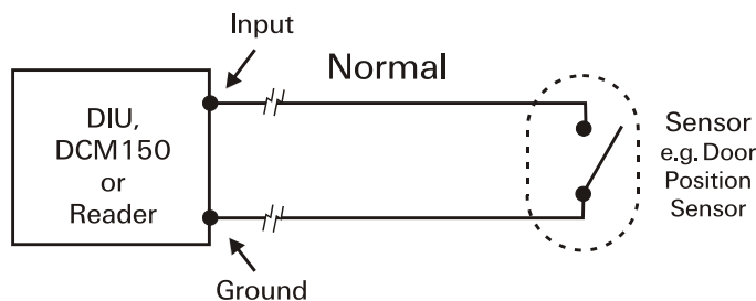
Normal Input sensor monitoring Open and Closed Conditions.
