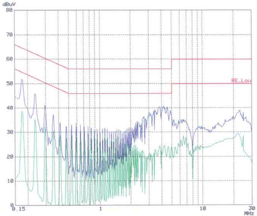
< Neutral line >
