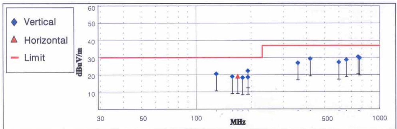
< Fig 6. Radiated emission result (Analog) >
