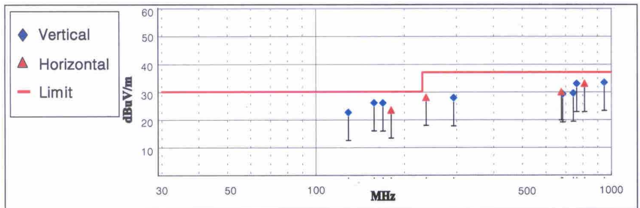
< Fig 7. Radiated emission result (Digital) >
