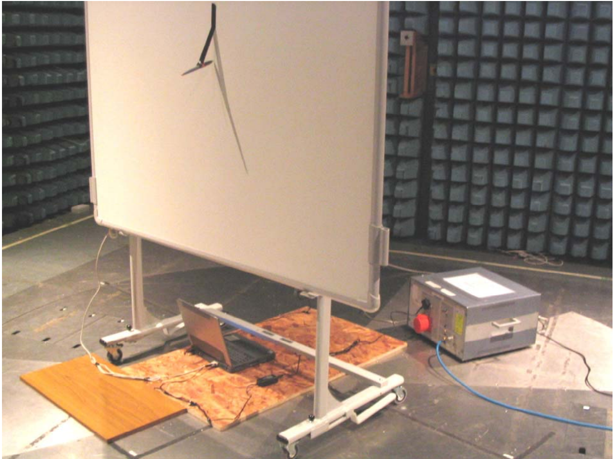
Conducted Emissions Set Up Photograph
