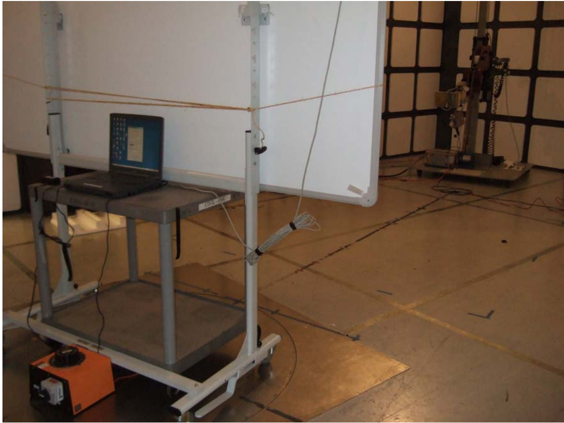
Radiated Emissions
