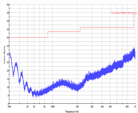
30MHz – 1GHz
