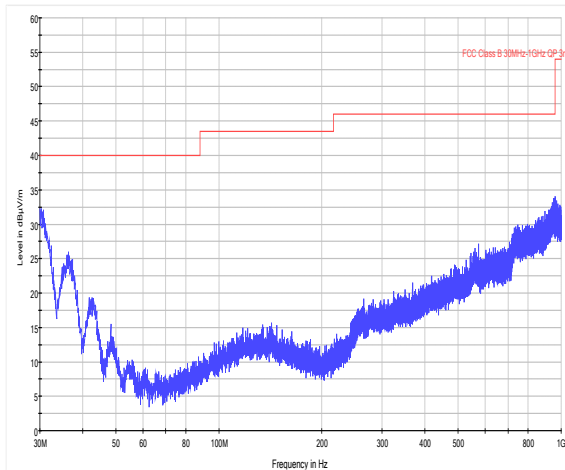
30MHz – 1GHz
