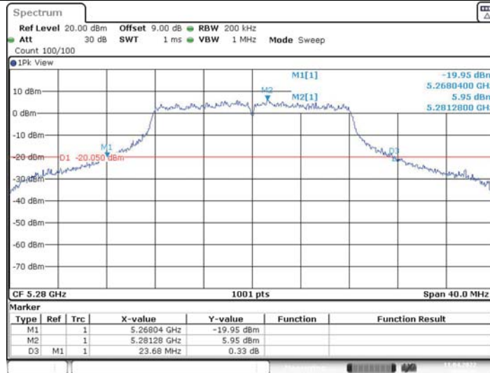
11A Ant2_5280
