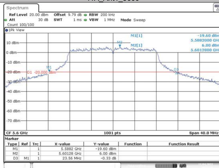
11A Ant1_5600
