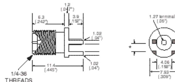
CONREVSMA003.031 for .031 Board Thickness CONREVSMA003.062 for .062 Board Thickness
