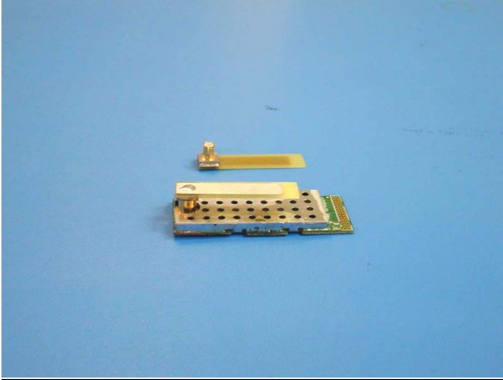
Photo 3 – PCB Patch Antenna
