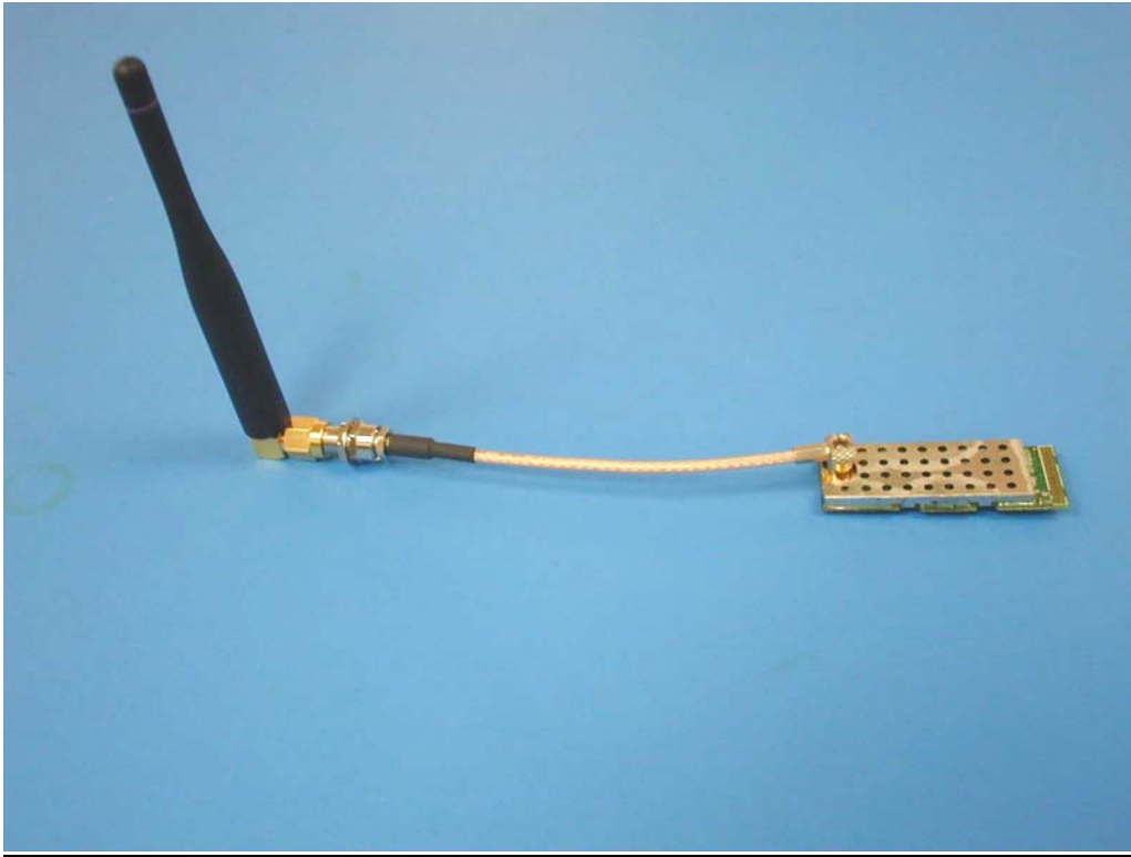
Photo 1 – Half Wavelength Dipole w/ 10 cm Cable
