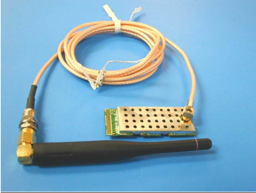
Photo 2 – Half Wavelength Dipole w/ 2m Cable
