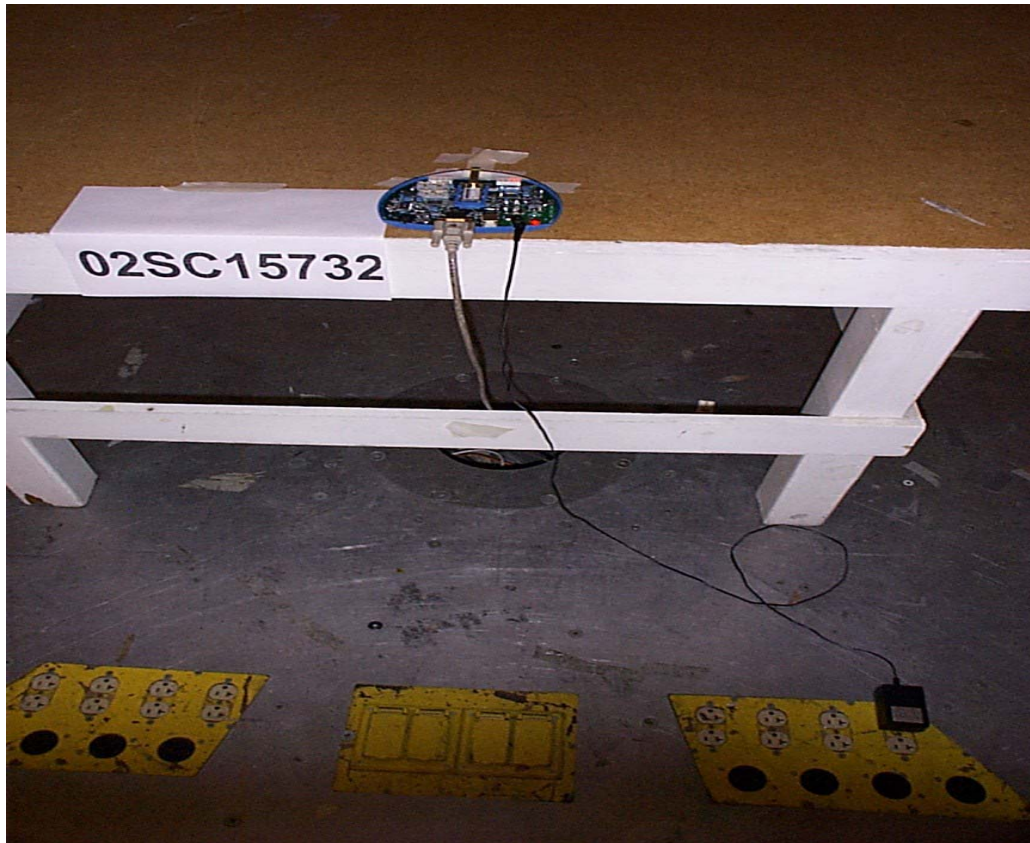
Photo 3 – Radiated Emission Testing at Open Area Test Site
