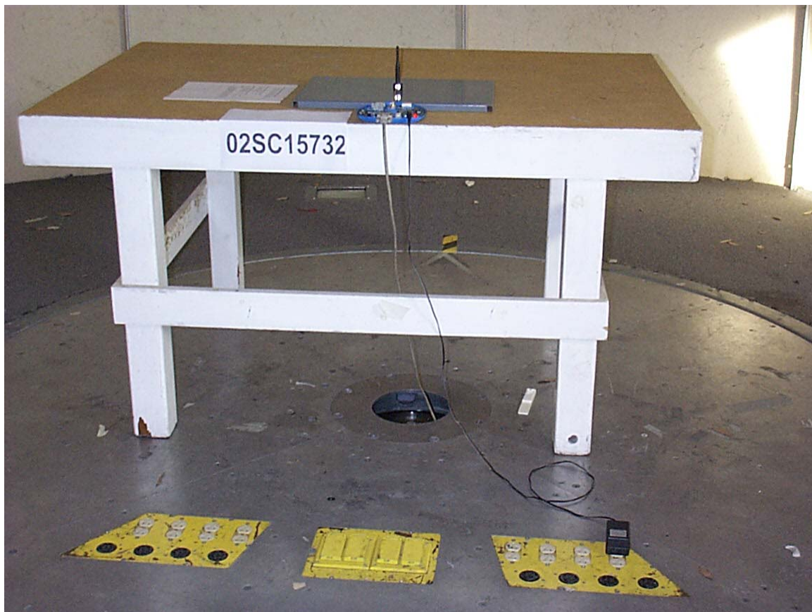
Photo 2 – Radiated Emission Testing at Open Area Test Site
