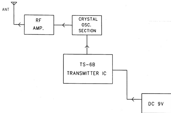
Remote Control Truck Transmitter BLOCK DIAGRAM
