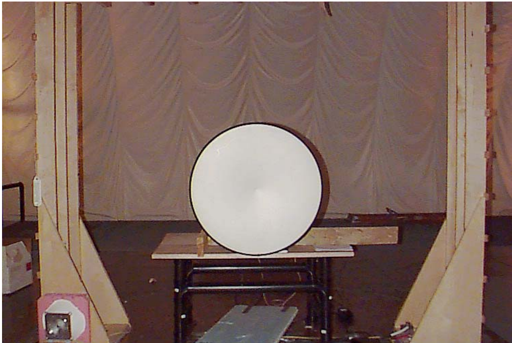
Large Antenna, 44.5dBi
