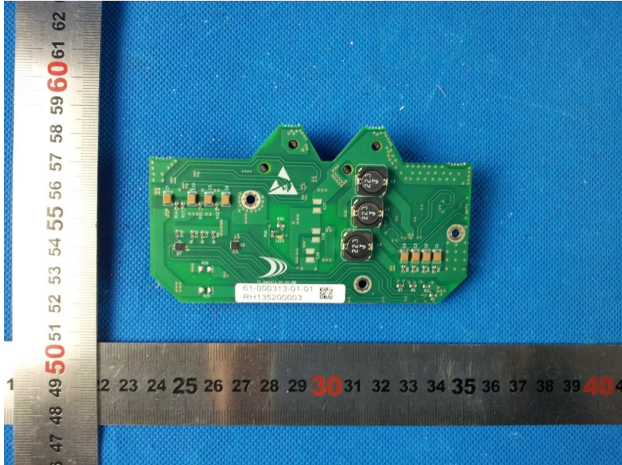
Photo 24 View of PoE+ daughter card
