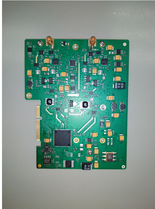
Photo 20 View of RF daughter card
