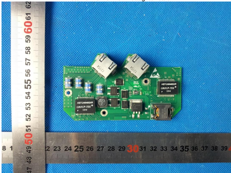
Photo 25 View of PoE+ daughter card
