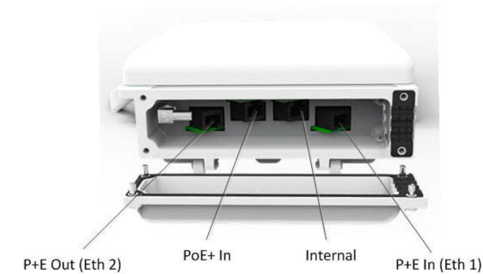
Figure 14 PoE+/P+E Interfaces
