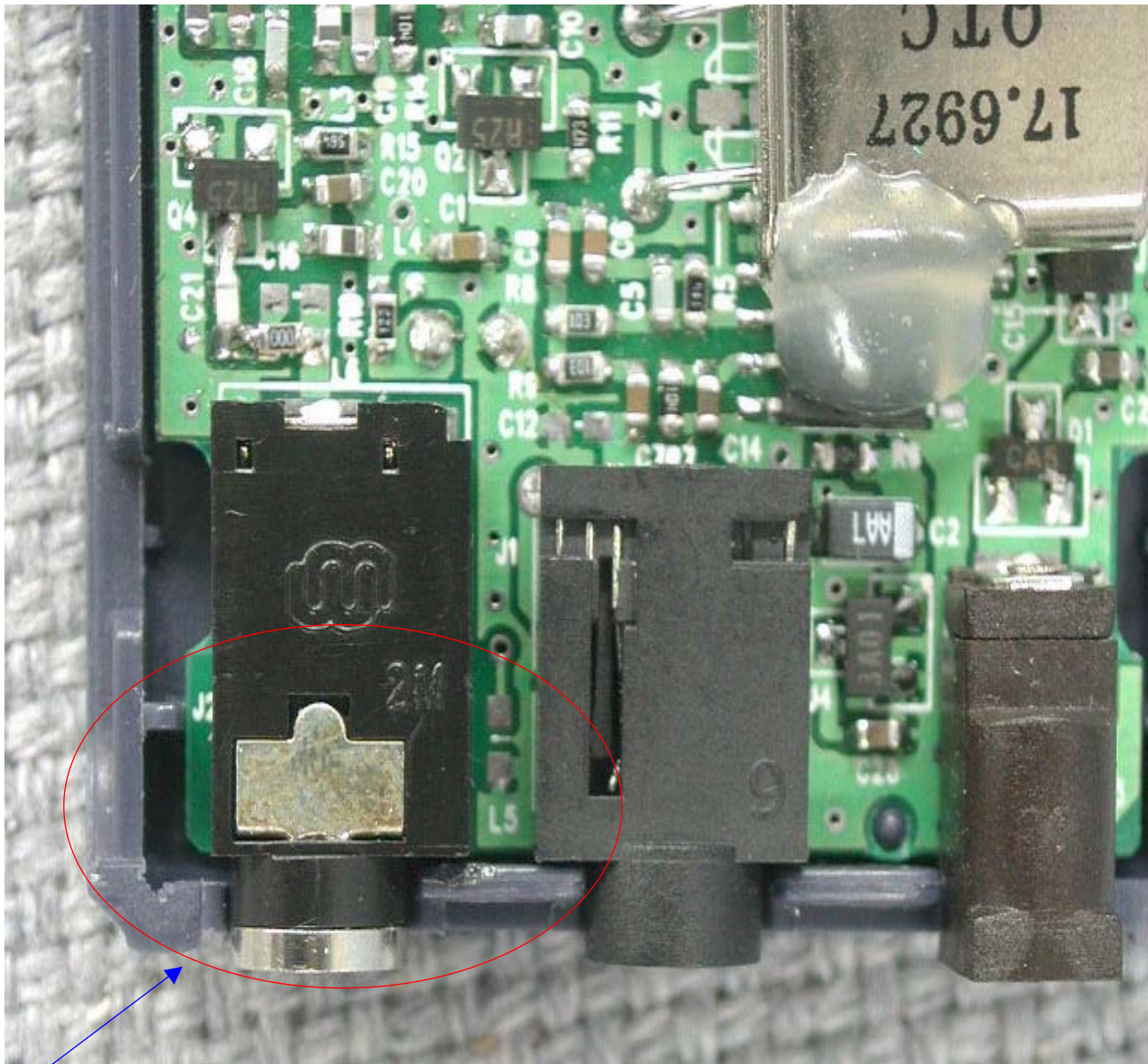
ANTENNA CONNECTOR
