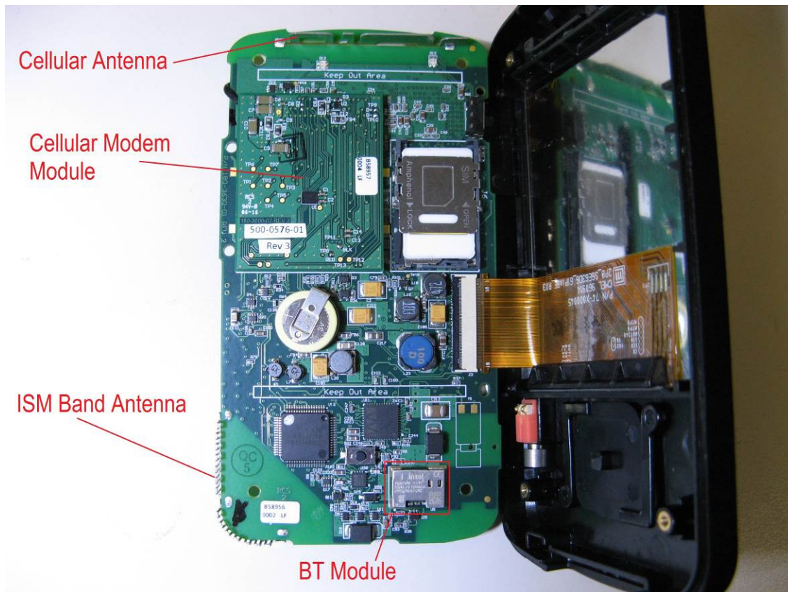
Figure 5: PCBA - Top view
