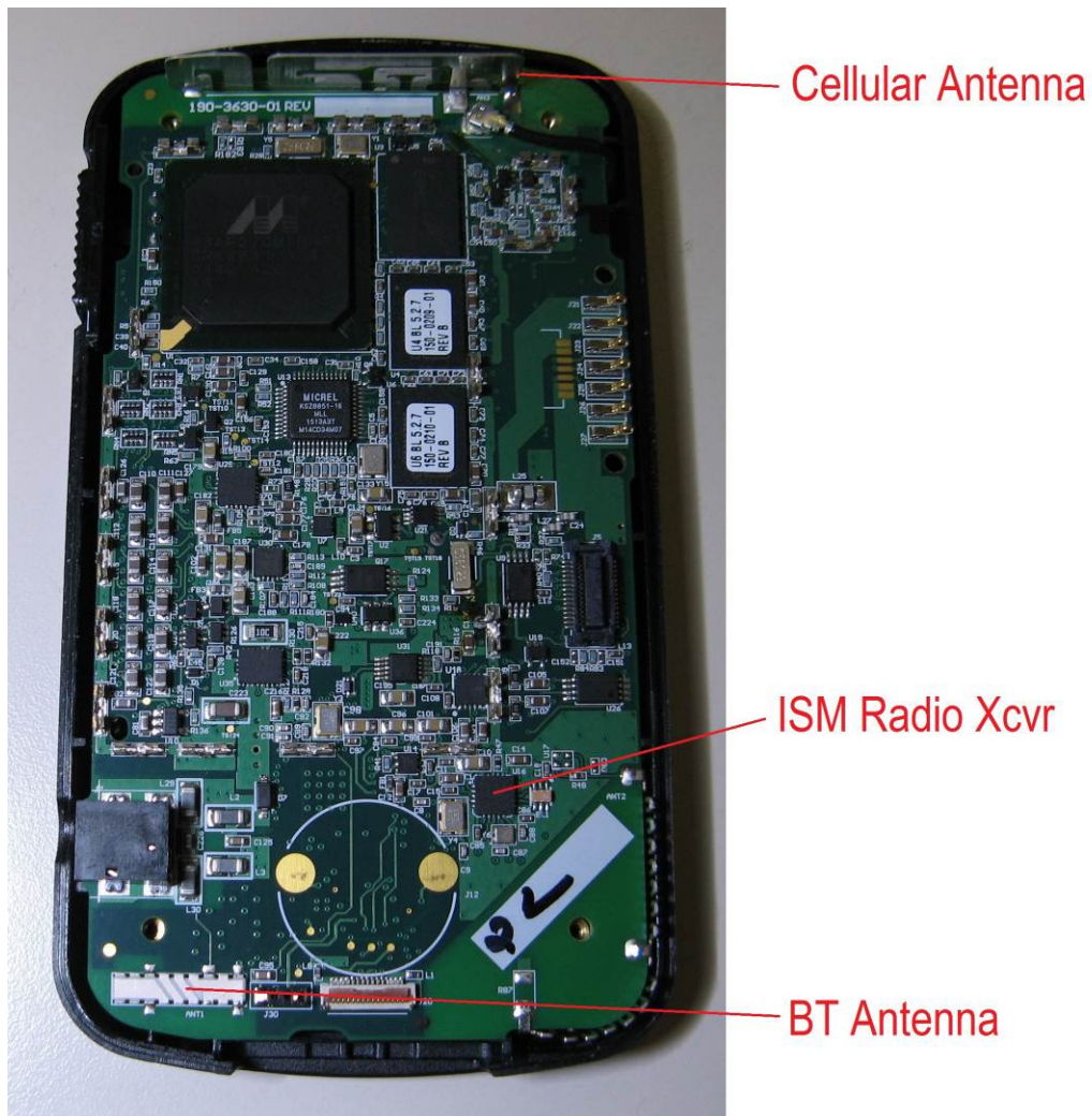
Figure 3: PCBA – Bottom view without shield
