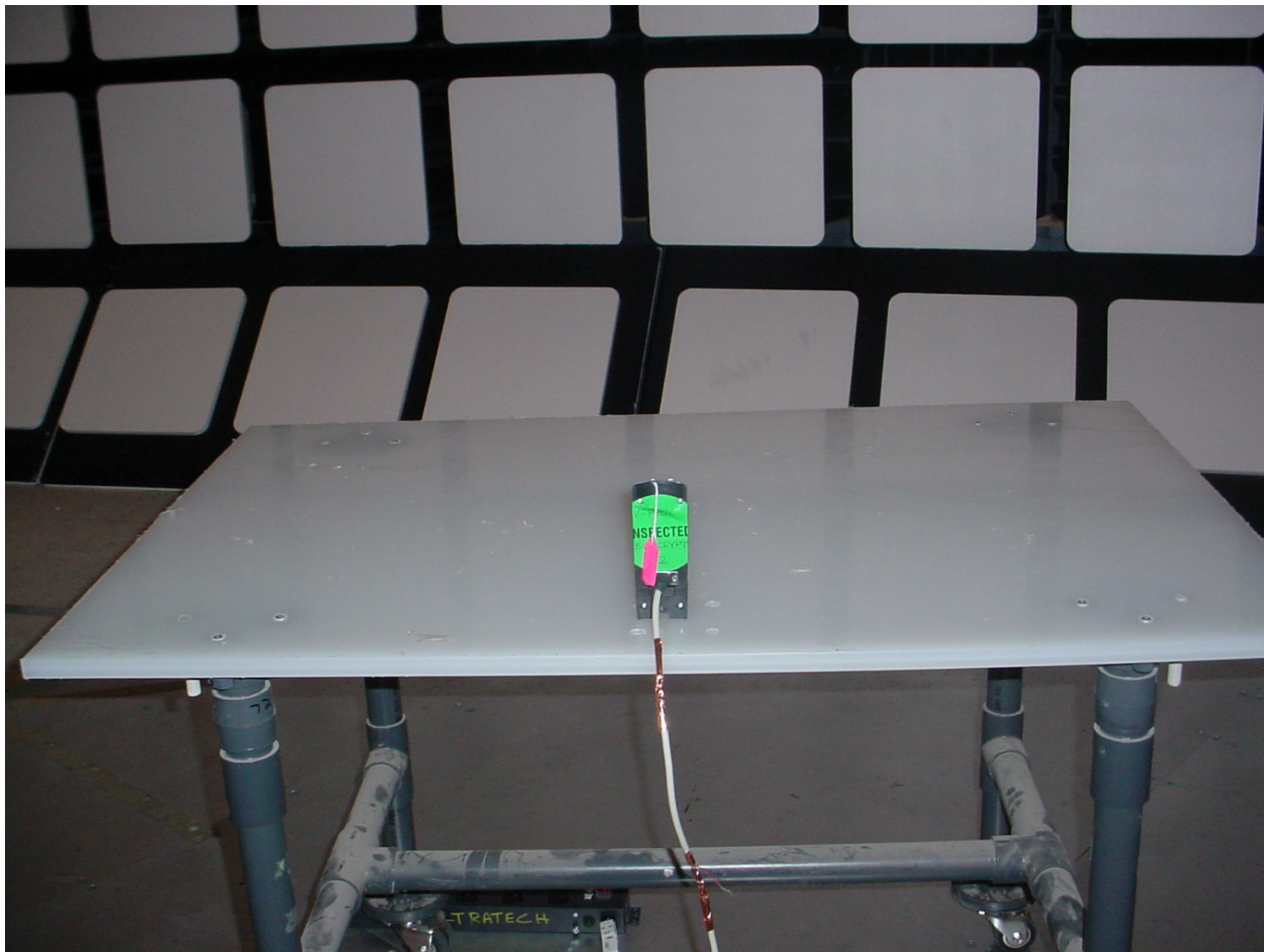
Photo #4: Radiated Emissions Measurements
