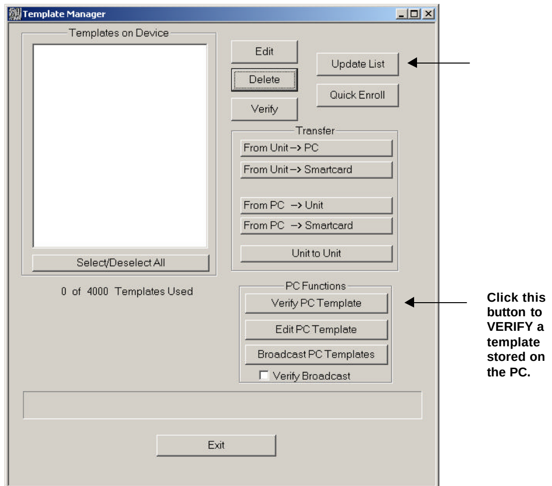
Figure 13: Template Manager
