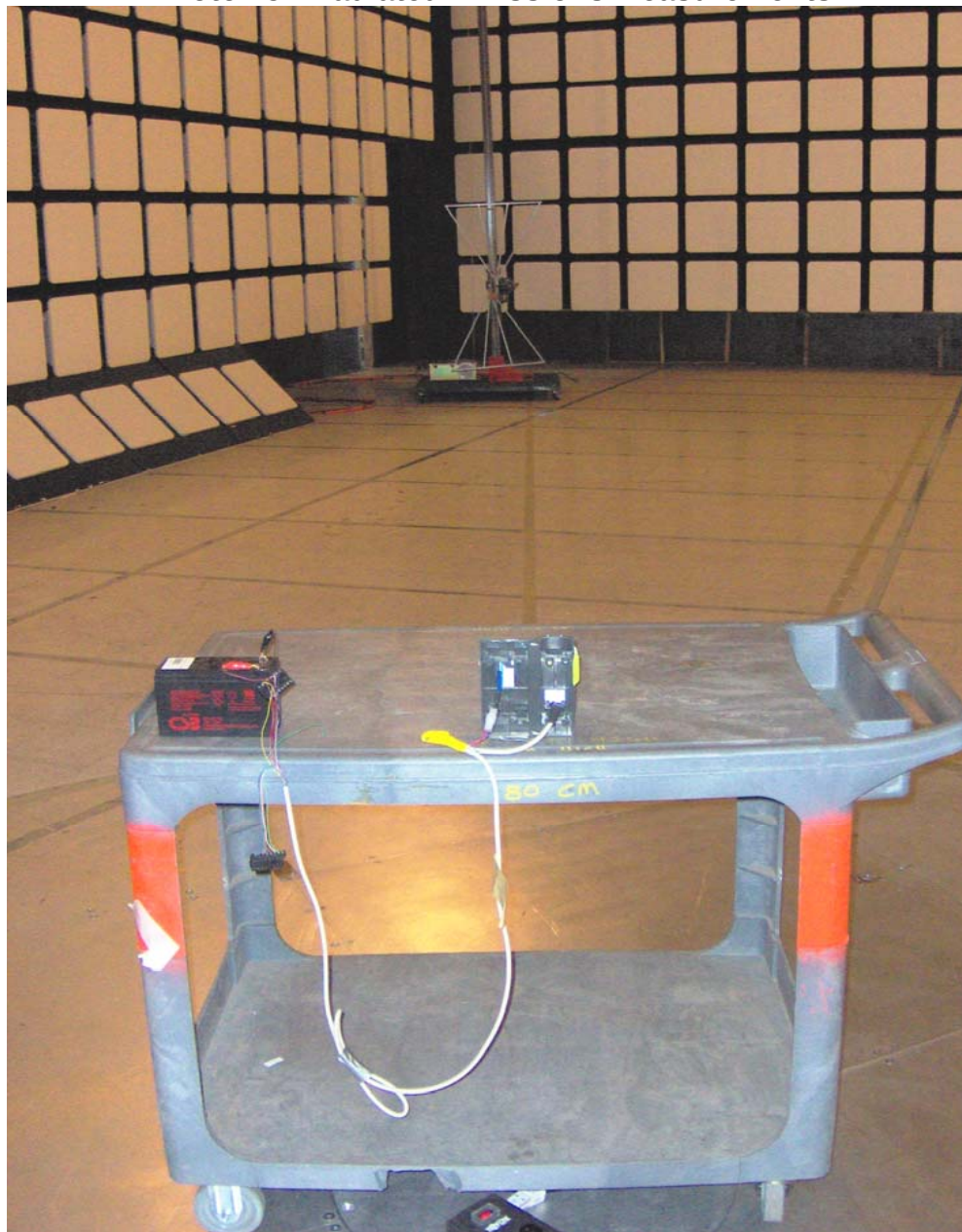
Photo #5: Radiated Emissions Measurements
