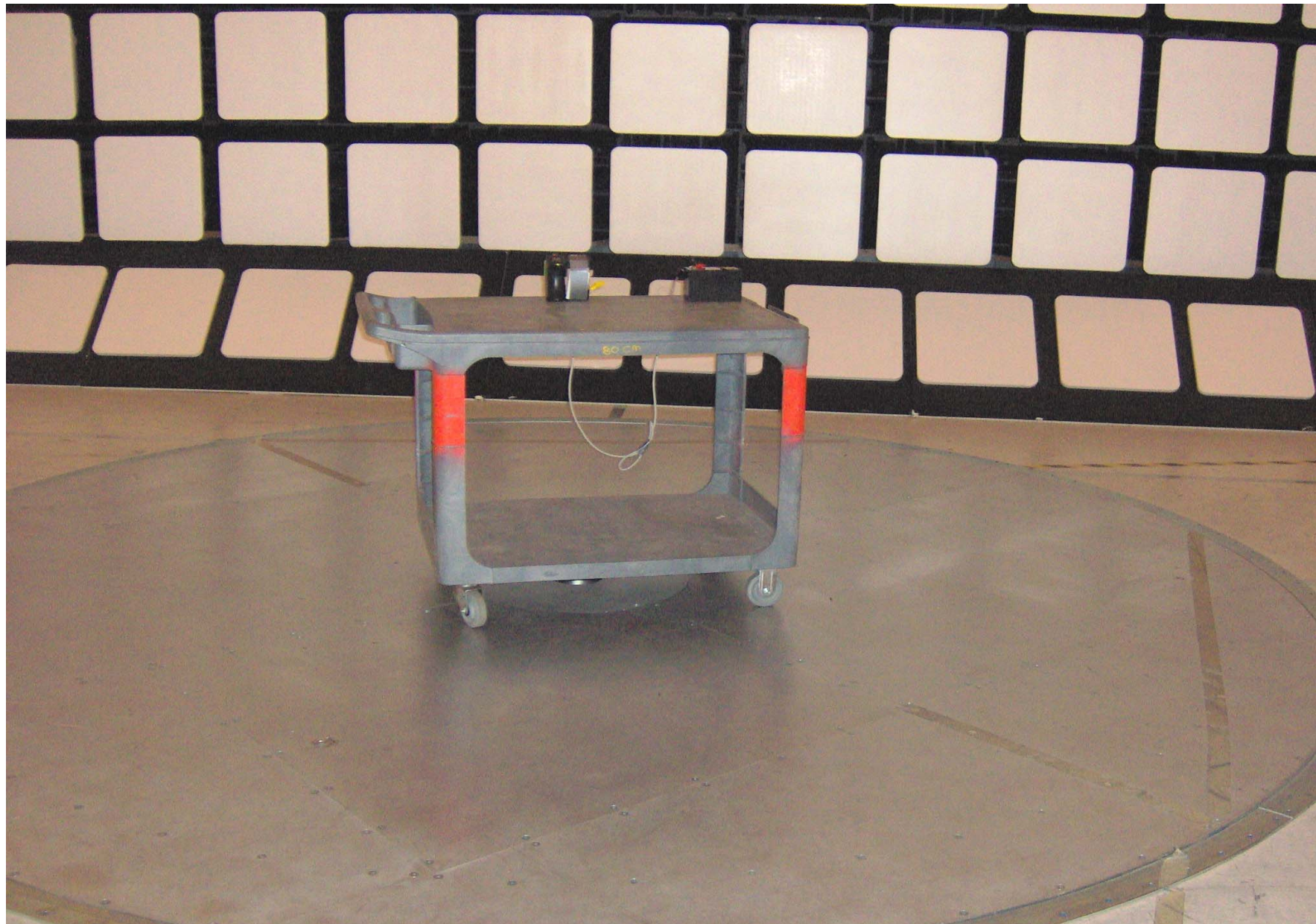
Photo #4: Radiated Emissions Measurements
