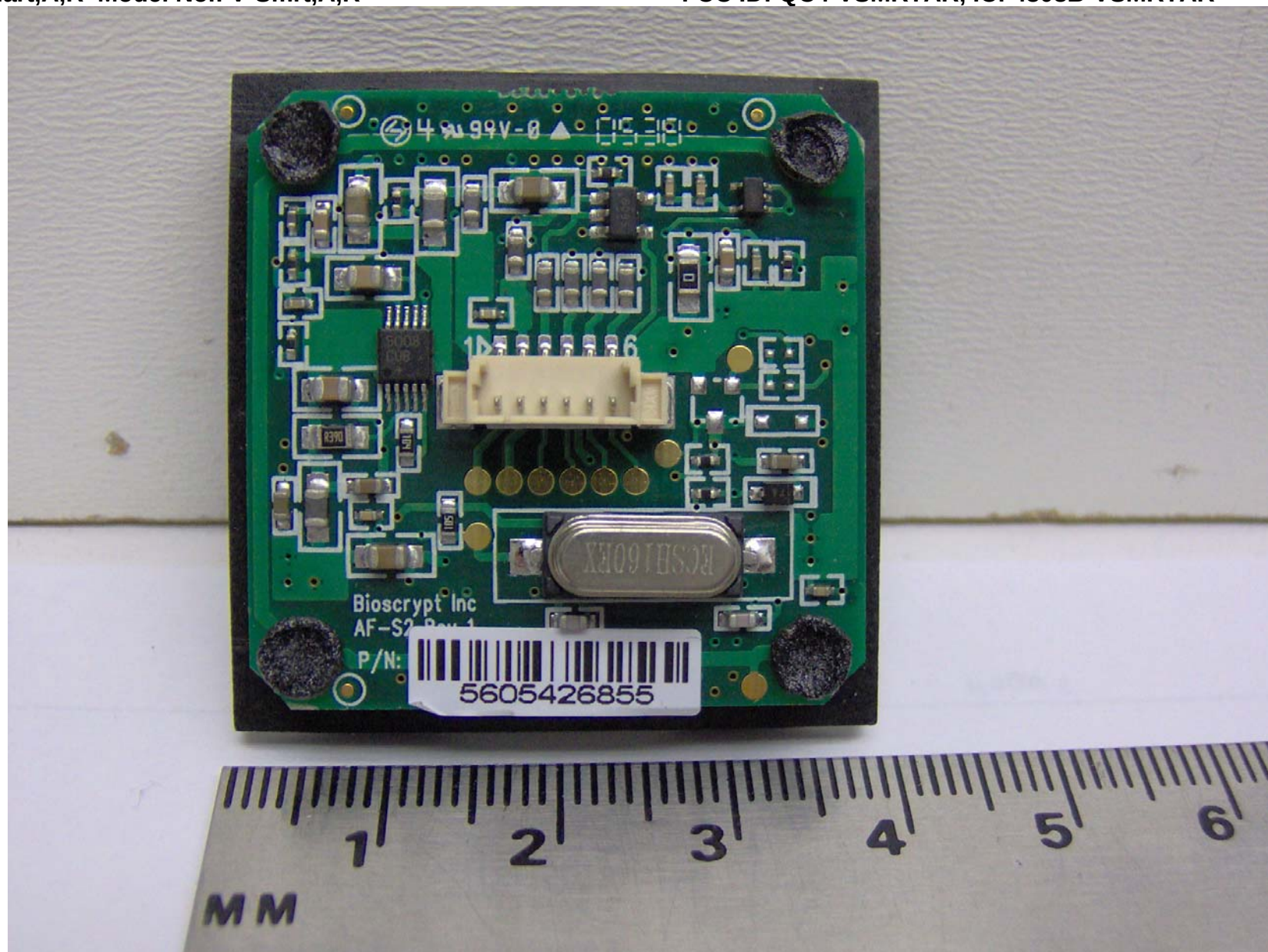
Annex 3: Internal Photographs of Device Under Test V-Smart,A,R Model No.: V-Smrt,A,R
