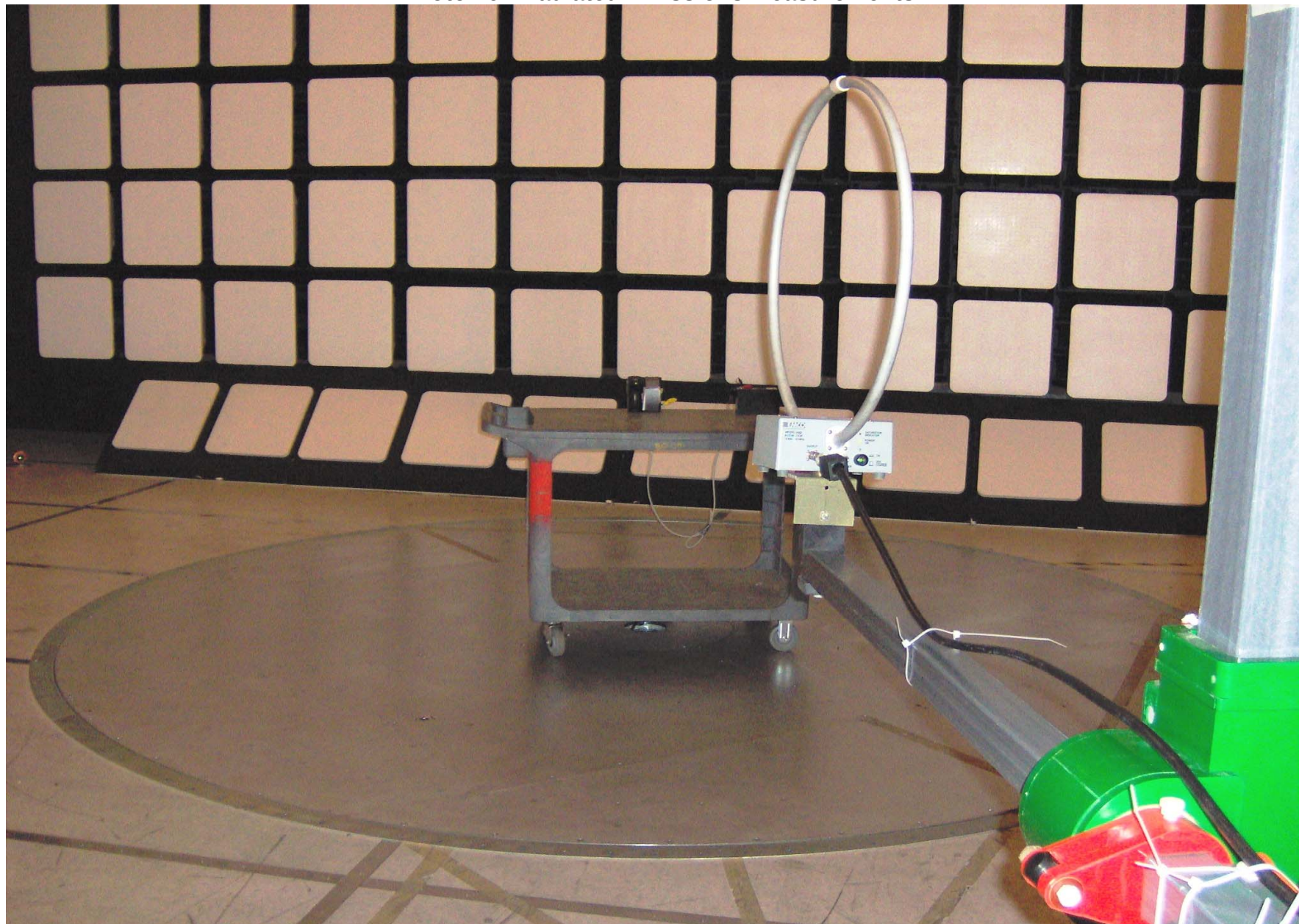
Photo #6: Radiated Emissions Measurements
