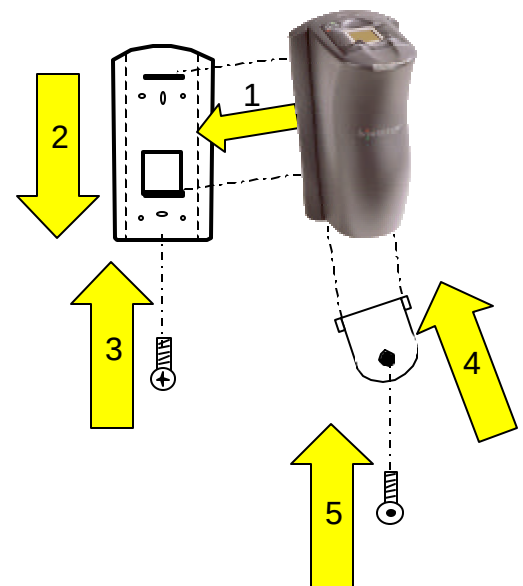
Figure 5: Mounting the reader to the wall
