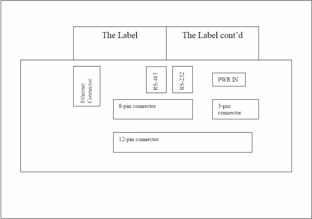
Rear view of V-Station (not to scale)
