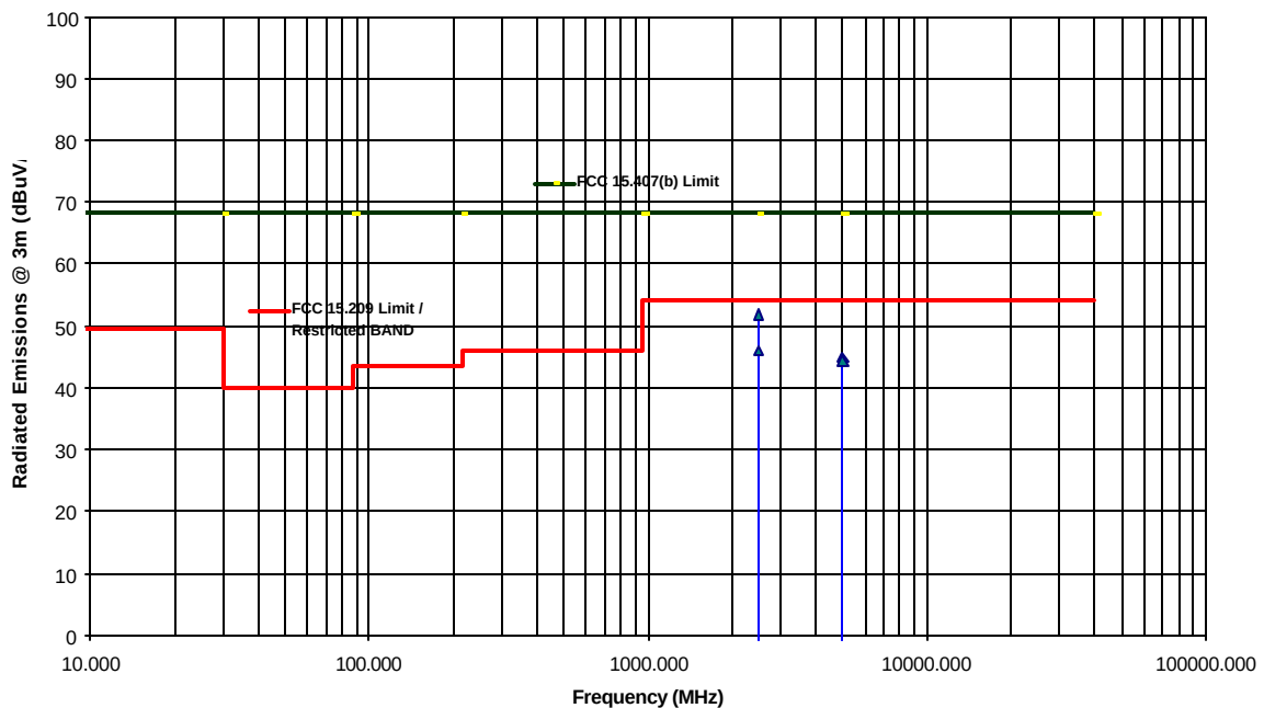
Transmitter Radiated Emissions Measurements at 3 Meter OFTS Redline Communications Inc. Access Node, Model AN-50, Tx Freq.: 5.815 GHz, RF Output Power: Maximum
