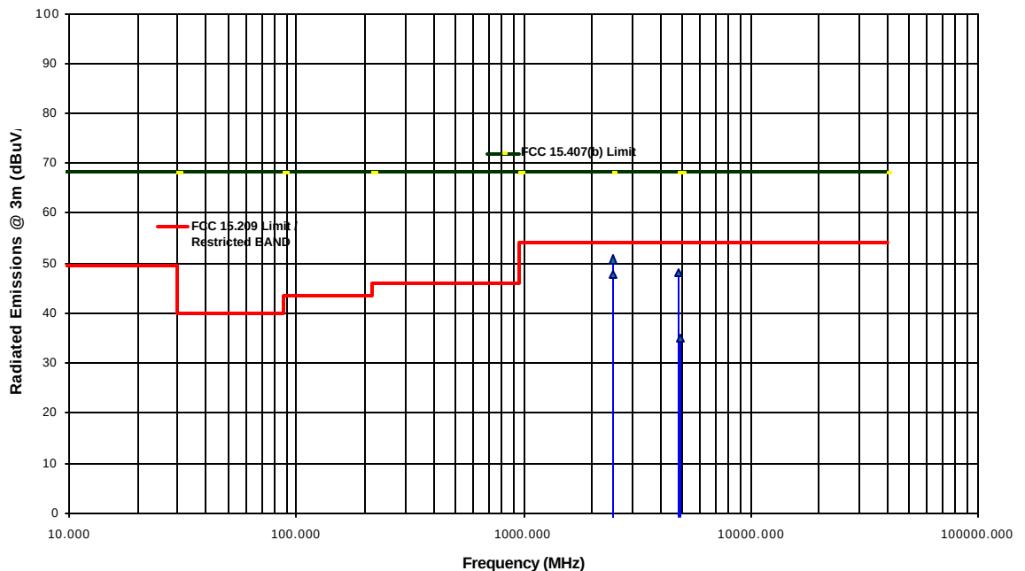
Transmitter Radiated Emissions Measurements at 3 Meter OFTS Redline Communications Inc. Access Node, Model AN-50, Tx Freq.: 5.725 GHz, RF Ouput Power: Maximum
