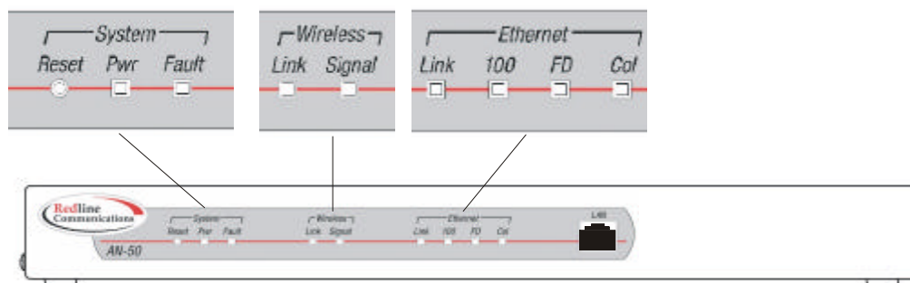
Figure 20 Front panel status LEDs.
