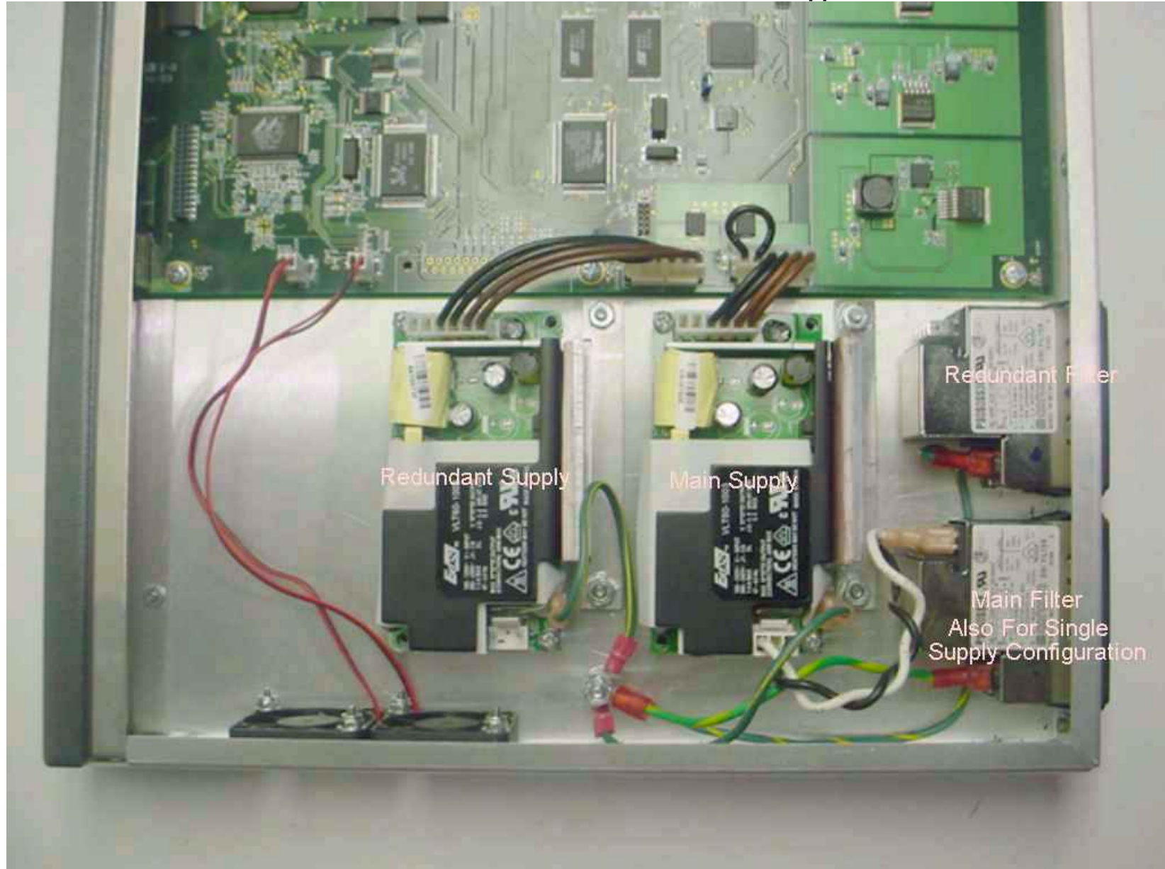
Model AN-50e / AN-30e with Dual AC Power Supplies
