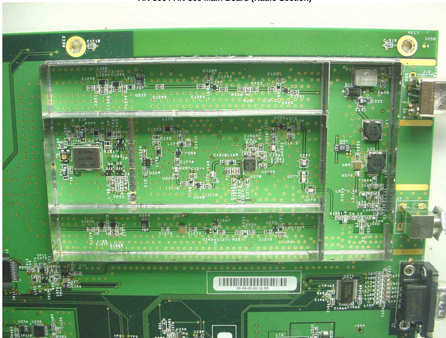
AN-50e / AN-30e Main Board (Radio Section)
