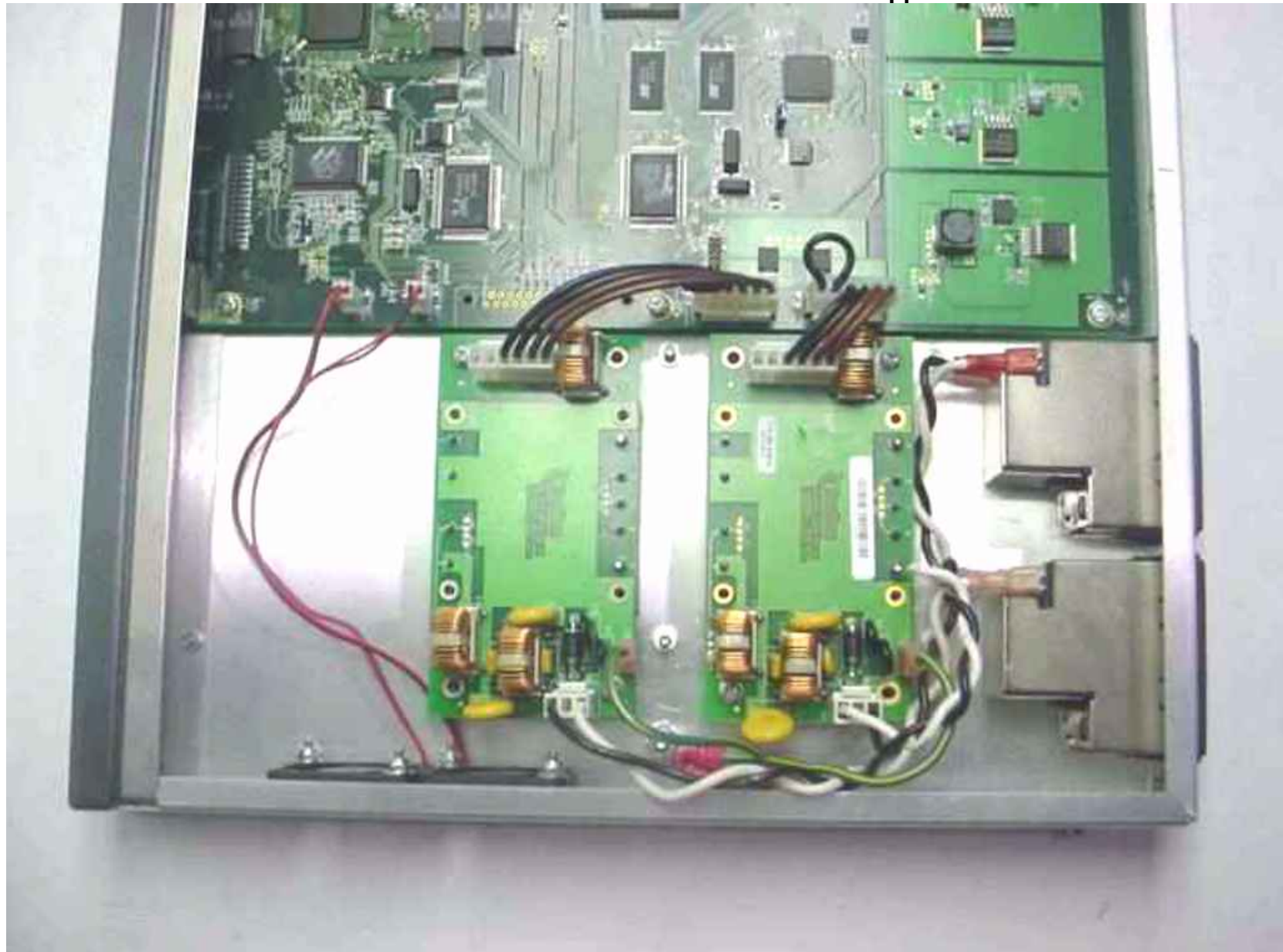
Model AN-50e / AN-30e with DC & DC Power Supplies
