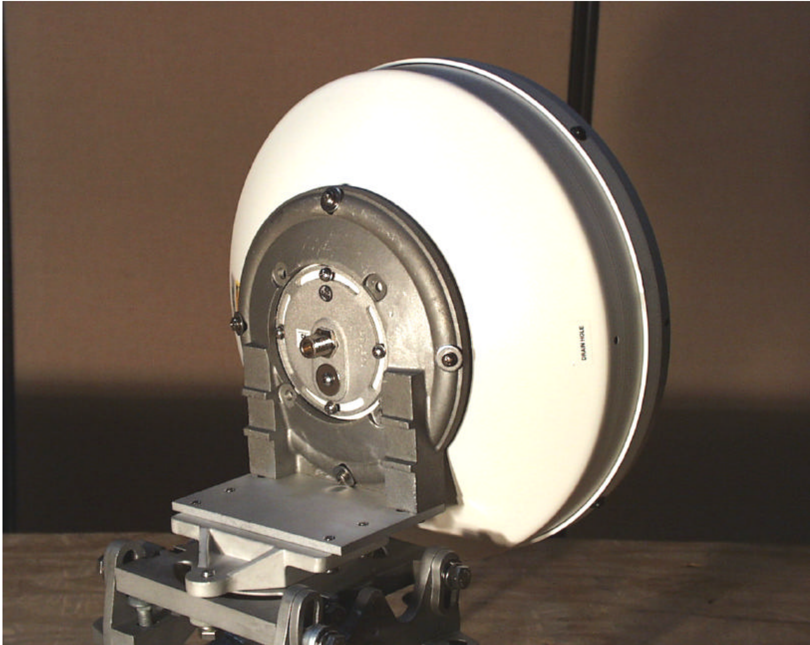
Radiowave Antenna, P/N: SP1-5.2NS, Gain 22.5 dBi (Back)
