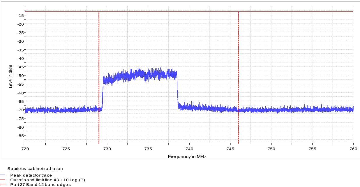
Figure 8.3-9: Radiated spurious emission at the lower band edge, 10 MHz channel, 16-QAM
