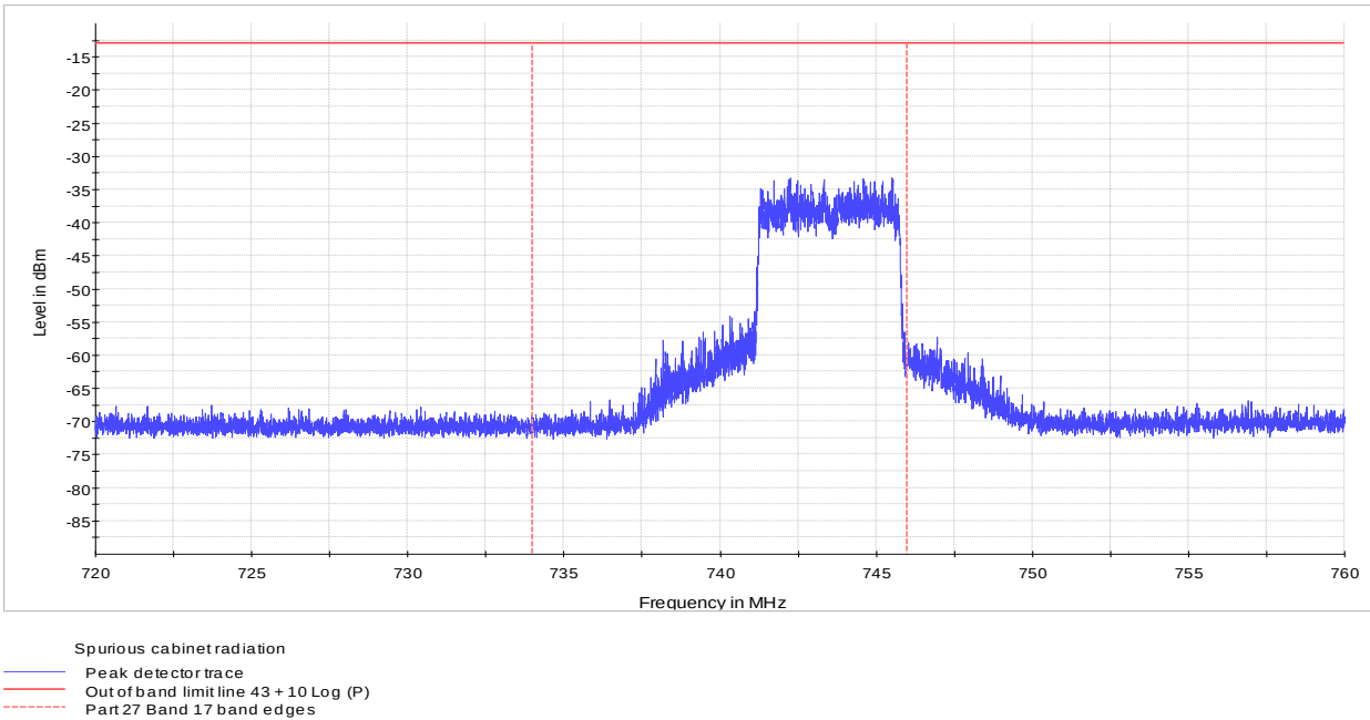
Figure 8.7-12: Radiated spurious emission at the upper band edge, 5 MHz channel, 16-QAM
