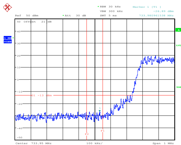
Figure 8.6-37: Lower band edge emission, 5 MHz channel, antenna 1
