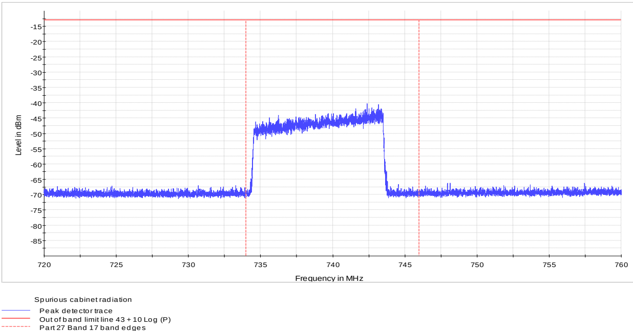
Figure 8.7-10: Radiated spurious emission at the lower band edge, 10 MHz channel, 64-QAM
