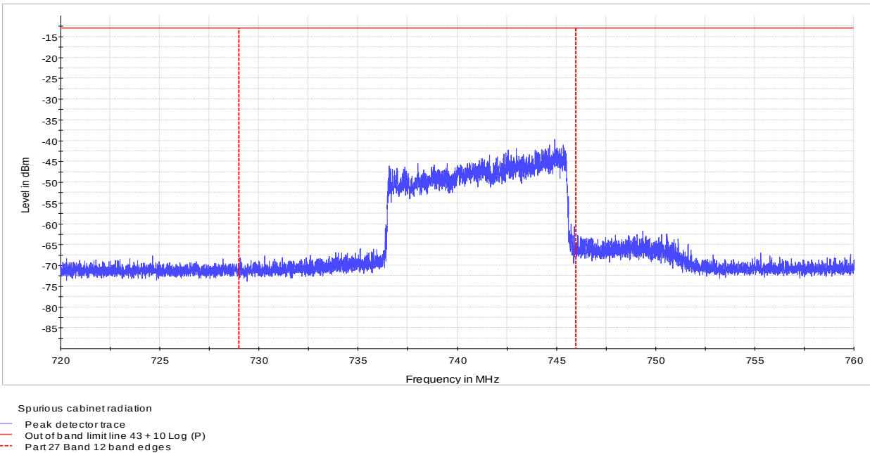
Figure 8.3-15: Radiated spurious emission at the upper band edge, 10 MHz channel, 16-QAM
