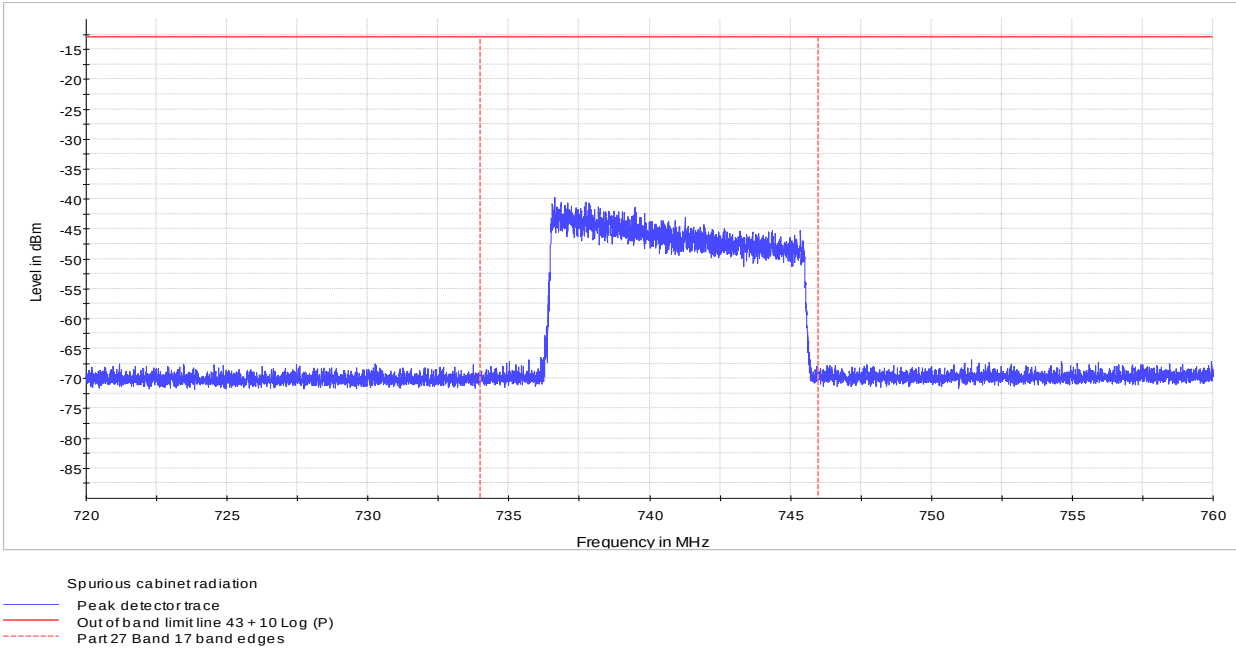
Figure 8.7-16: Radiated spurious emission at the upper band edge, 10 MHz channel, 64-QAM
