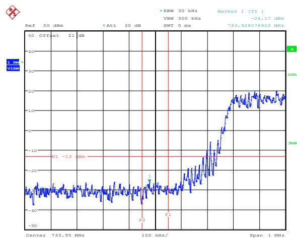
Figure 8.6-38: Lower band edge emission, 5 MHz channel, antenna 2
