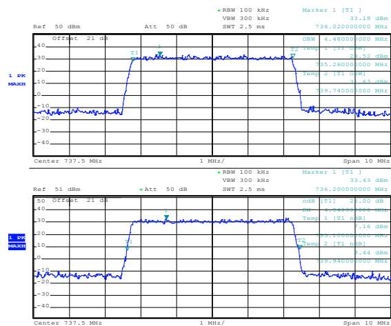
Figure 8.4-3: Occupied bandwidth, 5 MHz channel, 16-QAM, antenna 1
