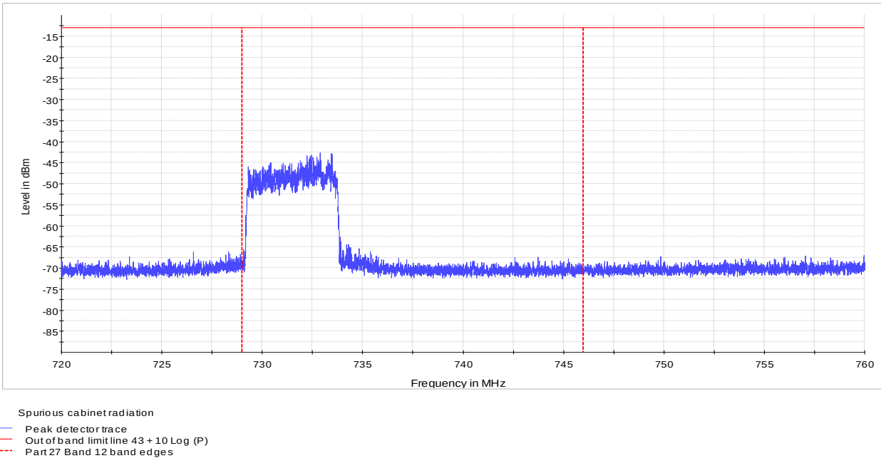
Figure 8.3-6: Radiated spurious emission at the lower band edge, 5 MHz channel, 16-QAM
