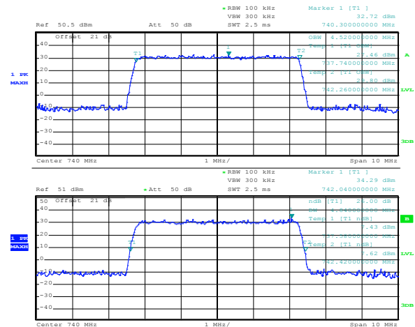
Figure 8.8-4: Occupied bandwidth, 5 MHz channel, 16-QAM, antenna 2
