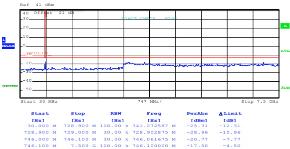
Figure 8.2-13: Conducted spurious emissions, antenna 1, 5 MHz, low channel, 64-QAM
