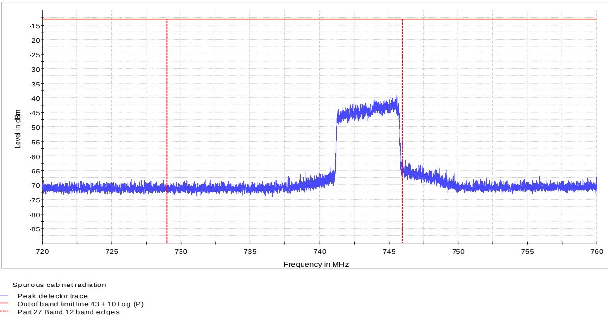
Figure 8.3-12: Radiated spurious emission at the upper band edge, 5 MHz channel, 16-QAM
