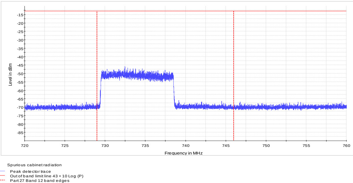
Figure 8.3-10: Radiated spurious emission at the lower band edge, 10 MHz channel, 64-QAM
