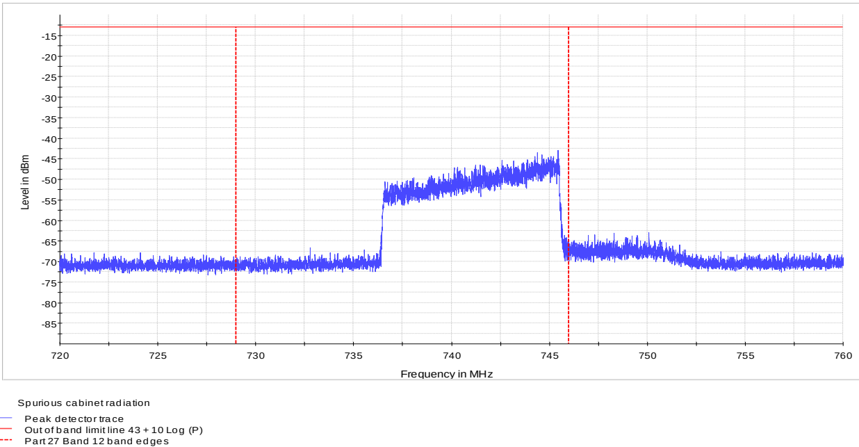
Figure 8.3-16: Radiated spurious emission at the upper band edge, 10 MHz channel, 64-QAM
