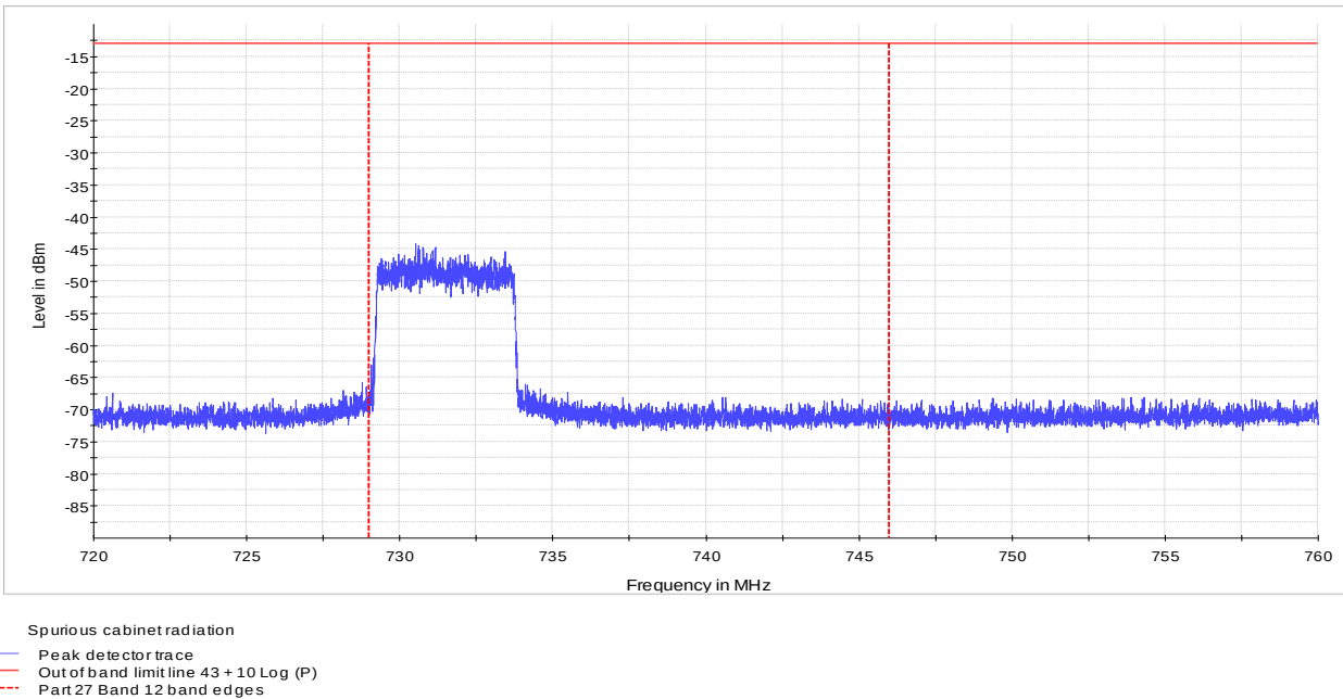
Figure 8.3-5: Radiated spurious emission at the lower band edge, 5 MHz channel, QPSK
