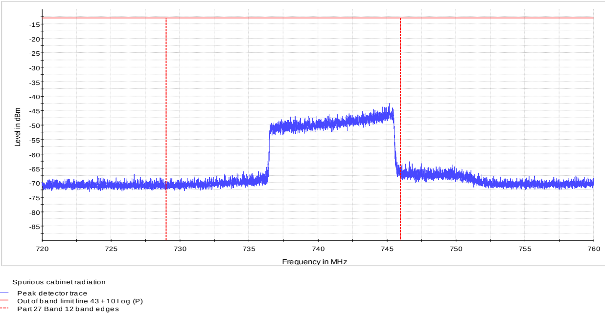
Figure 8.3-14: Radiated spurious emission at the upper band edge, 10 MHz channel, QPSK
