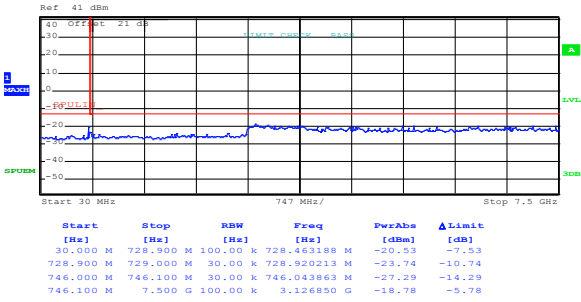
Figure 8.2-17: Conducted spurious emissions, antenna 2, 5 MHz, mid channel, 64-QAM
