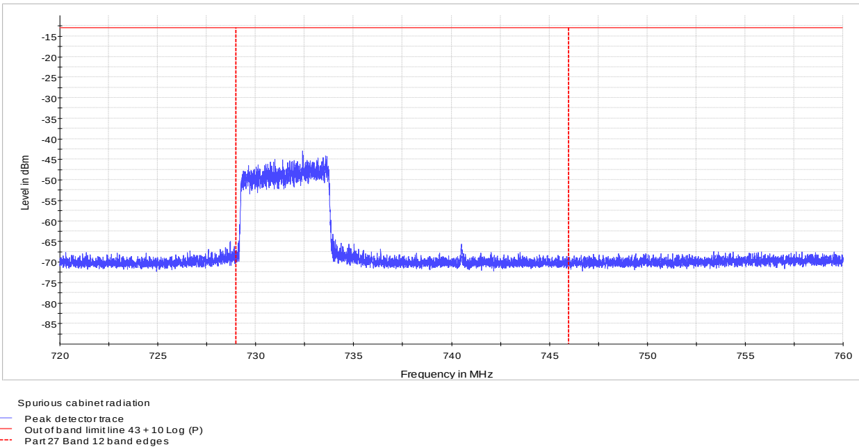
Figure 8.3-7: Radiated spurious emission at the lower band edge, 5 MHz channel, 64-QAM
