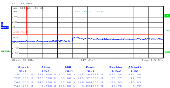
Figure 8.2-9: Conducted spurious emissions, antenna 1, 5 MHz, high channel, 16-QAM
