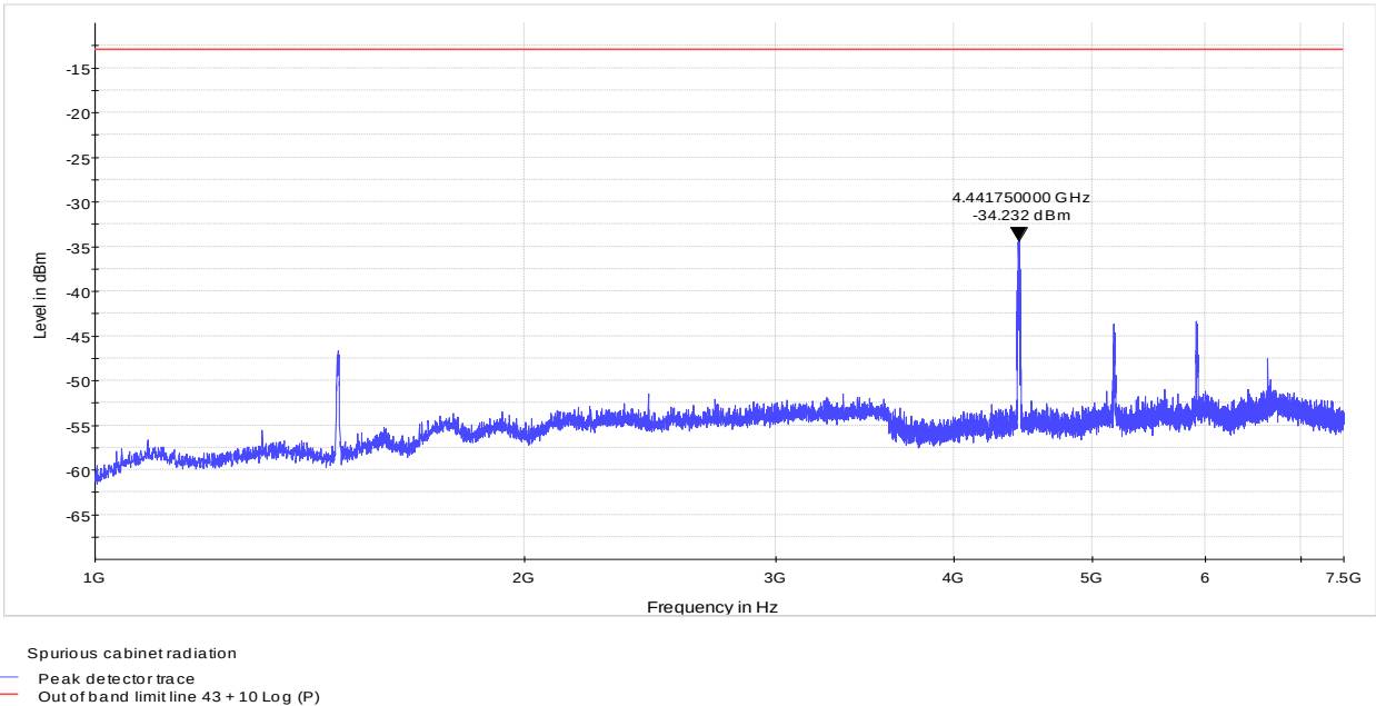
Figure 8.7-3: Radiated spurious emission above 1 GHz, 5 MHz channel
