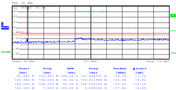
Figure 8.6-17: Conducted spurious emissions, antenna 2, 5 MHz, mid channel, 64-QAM
