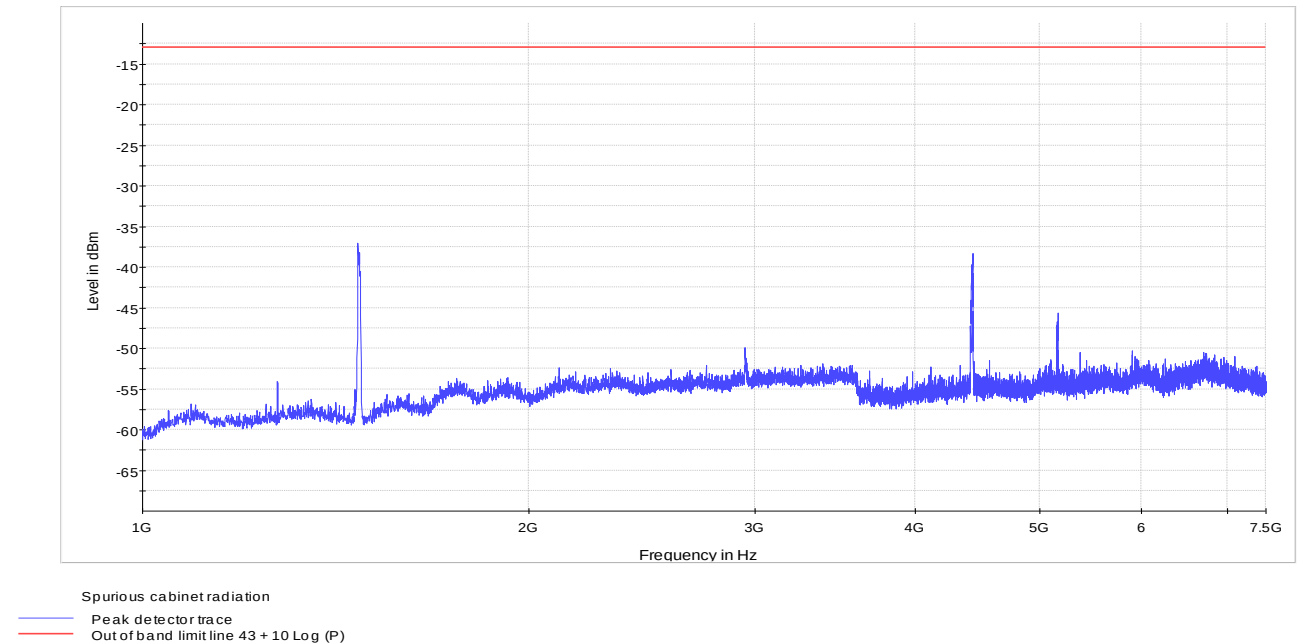
Figure 8.3-3: Radiated spurious emission above 1 GHz, 5 MHz channel
