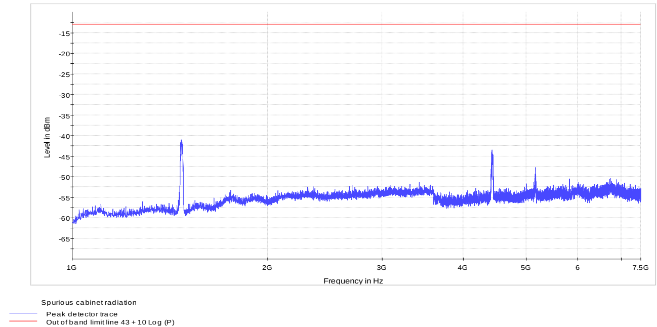
Figure 8.3-4: Radiated spurious emission above 1 GHz, 10 MHz channel
