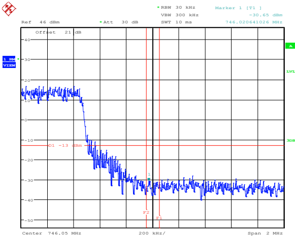
Figure 8.2-50: Upper band edge emission, 10 MHz channel, antenna 2
