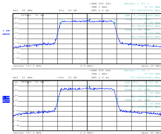
Figure 8.4-7: Occupied bandwidth, 10 MHz channel, QPSK, antenna 1
