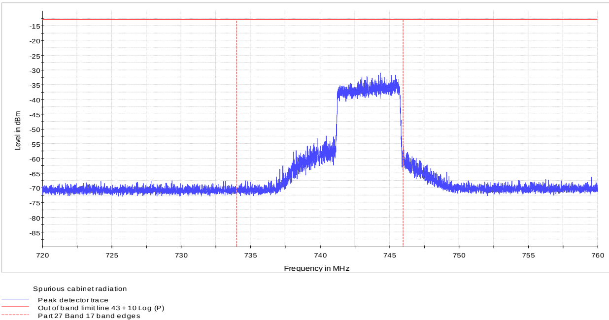
Figure 8.7-13: Radiated spurious emission at the upper band edge, 5 MHz channel, 64-QAM
