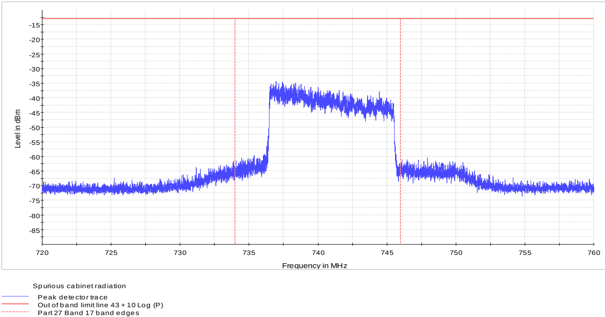
Figure 8.7-15: Radiated spurious emission at the upper band edge, 10 MHz channel, 16-QAM
