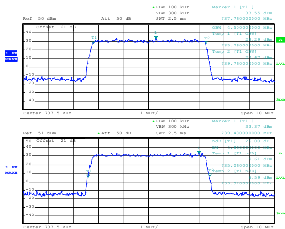
Figure 8.4-4: Occupied bandwidth, 5 MHz channel, 16-QAM, antenna 2
