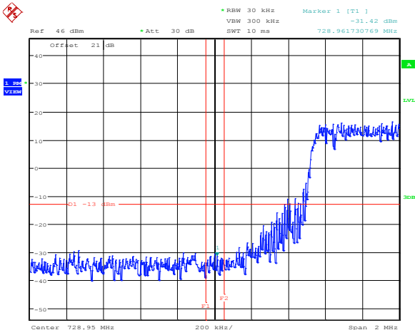
Figure 8.2-42: Lower band edge emission, 10 MHz channel, antenna 2
