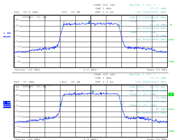
Figure 8.8-8: Occupied bandwidth, 10 MHz channel, QPSK, antenna 2
