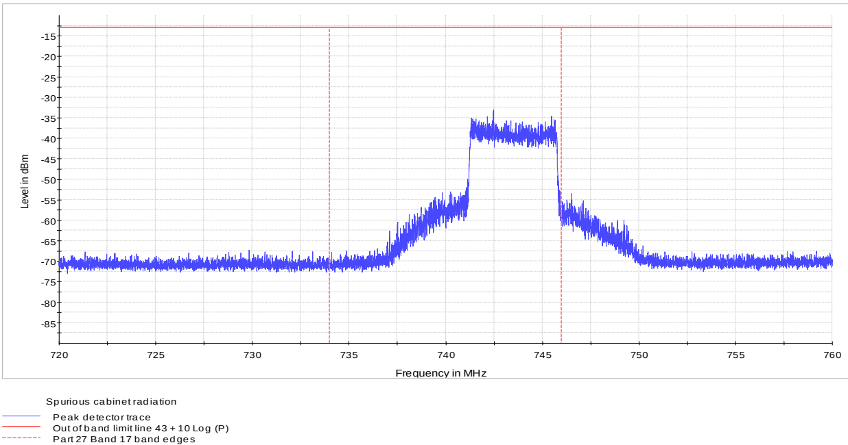
Figure 8.7-11: Radiated spurious emission at the upper band edge, 5 MHz channel, QPSK
