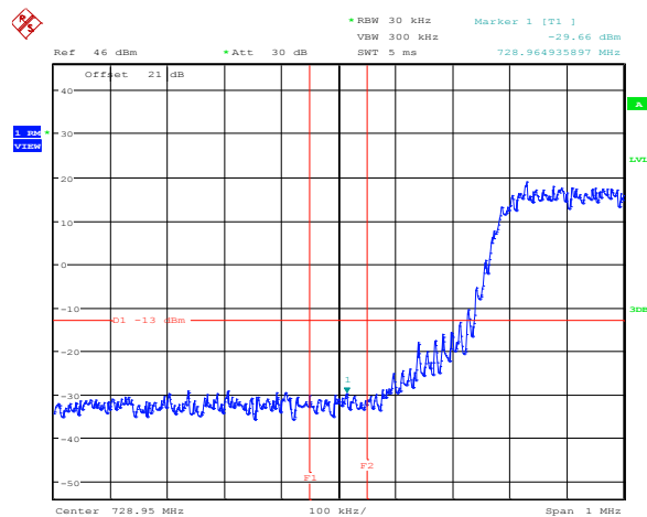
Figure 8.2-37: Lower band edge emission, 5 MHz channel, antenna 1
