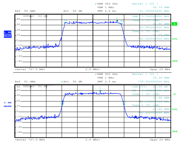
Figure 8.4-8: Occupied bandwidth, 10 MHz channel, QPSK, antenna 2
