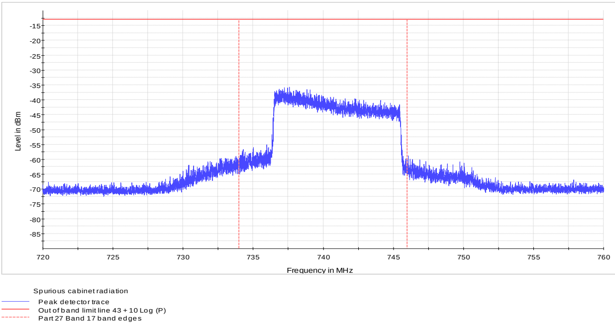
Figure 8.7-14: Radiated spurious emission at the upper band edge, 10 MHz channel, QPSK
