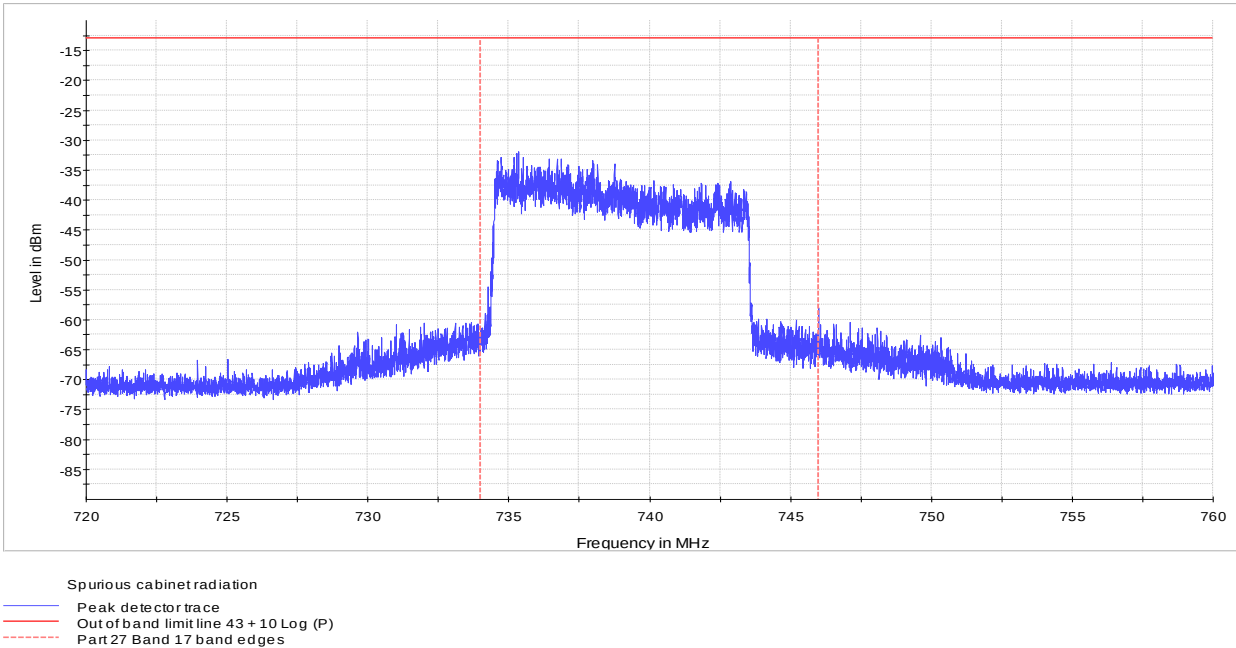
Figure 8.7-9: Radiated spurious emission at the lower band edge, 10 MHz channel, 16-QAM
