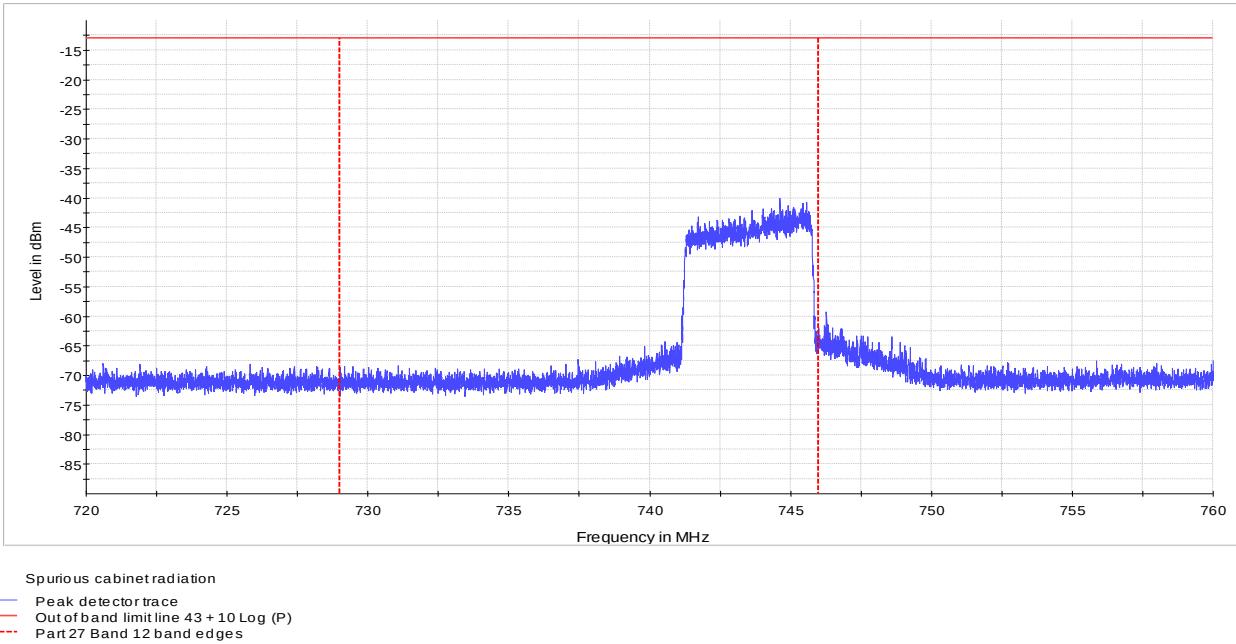
Figure 8.3-13: Radiated spurious emission at the upper band edge, 5 MHz channel, 64-QAM
