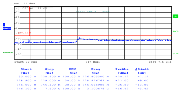
Figure 8.2-2: Conducted spurious emissions, antenna 1, 5 MHz, mid channel, QPSK
