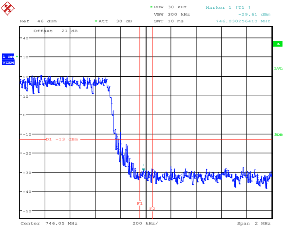
Figure 8.2-45: Upper band edge emission, 5 MHz channel, antenna 1
