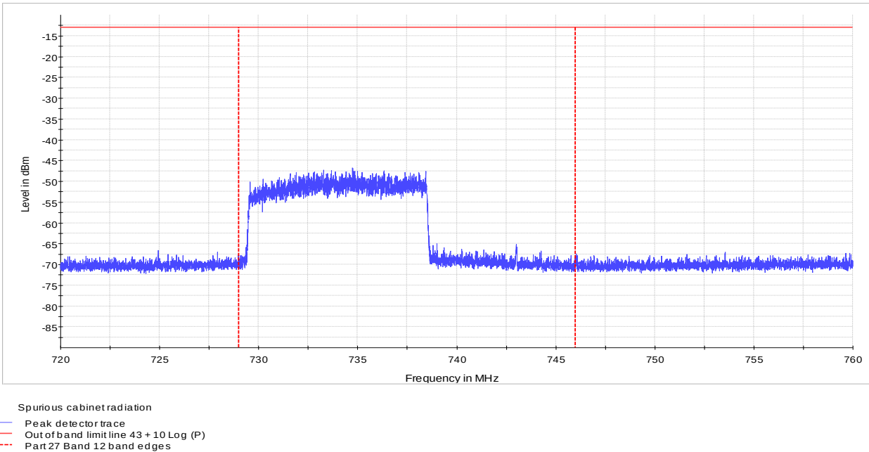
Figure 8.3-8: Radiated spurious emission at the lower band edge, 10 MHz channel, QPSK
