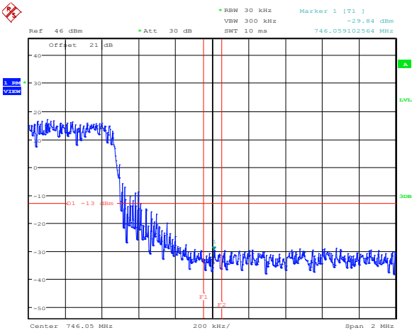
Figure 8.6-49: Upper band edge emission, 10 MHz channel, antenna 1
