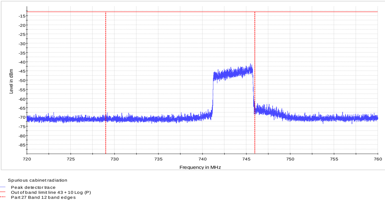
Figure 8.3-11: Radiated spurious emission at the upper band edge, 5 MHz channel, QPSK
