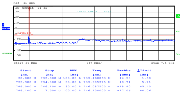
Figure 8.6-22: Conducted spurious emissions, antenna 1, 10 MHz, low channel, QPSK
