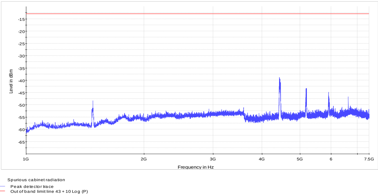
Figure 8.7-4: Radiated spurious emission above 1 GHz, 10 MHz channel
