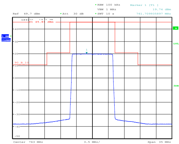
Figure 8.3-1: Emission mask at Ant 1, QPSK
