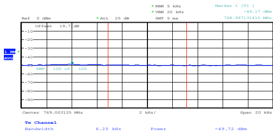
Figure 8.4-39: Conducted at the band edge at 769 MHz, Ant 1, 64-QAM
