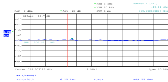
Figure 8.4-40: Conducted at the band edge at 769 MHz, Ant 2, QPSK
