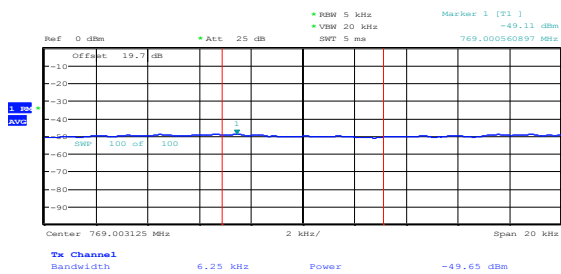
Figure 8.4-41: Conducted at the band edge at 769 MHz, Ant 2, 16-QAM
