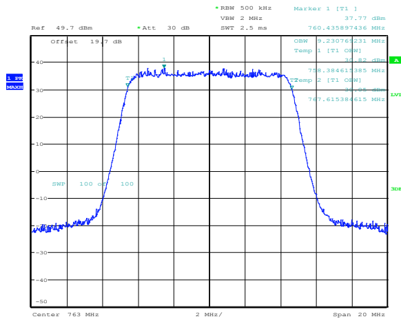
Figure 8.2-2: 99 % bandwidth Ant 1, 16-QAM
