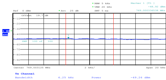
Figure 8.4-37: Conducted at the band edge at 769 MHz, Ant 1, QPSK
