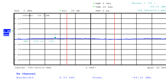
Figure 8.4-38: Conducted at the band edge at 769 MHz, Ant 1, 16-QAM
