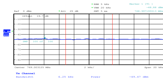
Figure 8.4-42: Conducted at the band edge at 769 MHz, Ant 2, 64-QAM
