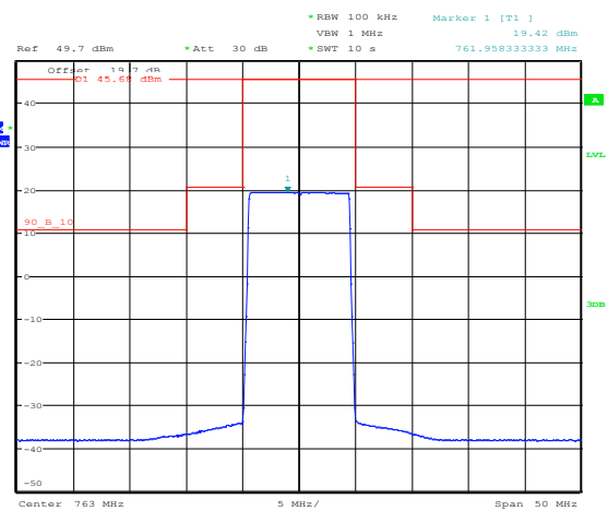
Figure 8.3-2: Emission mask at Ant 1, 16-QAM
