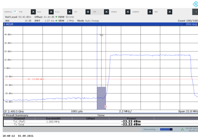
Figure 8.3-9: Band edge measurement for Ant 1 QPSK 10 MHz low channel
