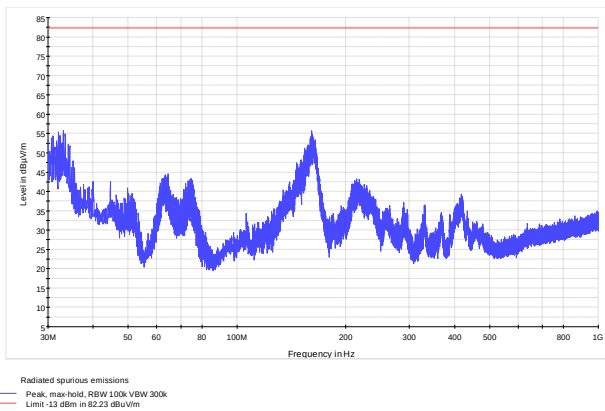
Figure 8.3-61 Cabinet spurious radiations 30–1000 MHz for low channel
