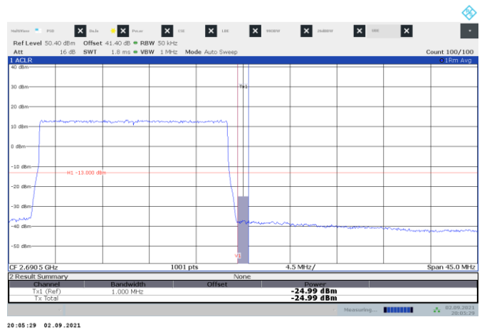
Figure 8.3-20: Band edge measurement for Ant 2 QPSK 20 MHz top channel
