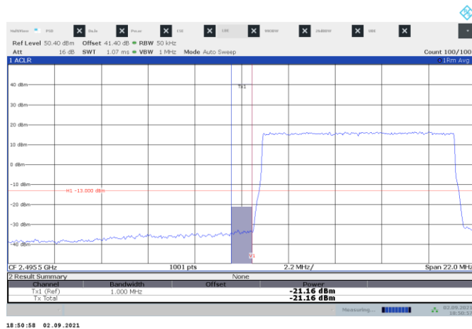
Figure 8.3-11: Band edge measurement for Ant 2 QPSK 10 MHz low channel
