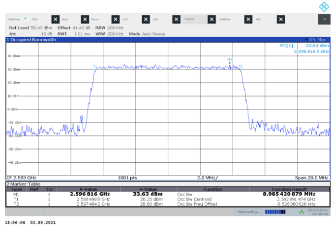
Figure 8.4-4: 99% OBW sample plot for 10 MHz channel
