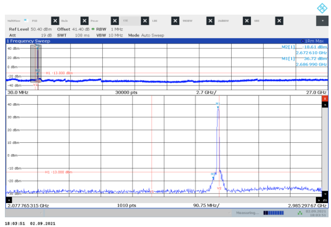
Figure 8.3-36: Conducted spurious emissions at Ant 2 64QAM 5 MHz top channel
