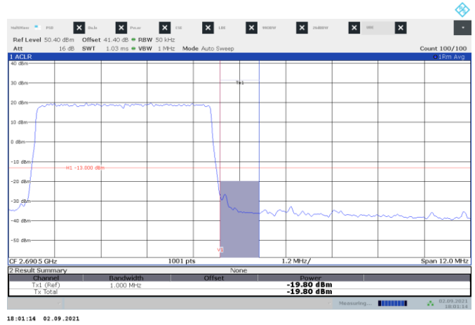
Figure 8.3-6: Band edge measurement for Ant 1 64QAM 5 MHz top channel
