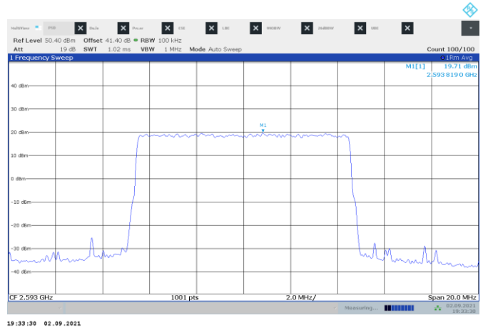
Figure 8.2-2: PSD for 10 MHz channel BW, sample plot
