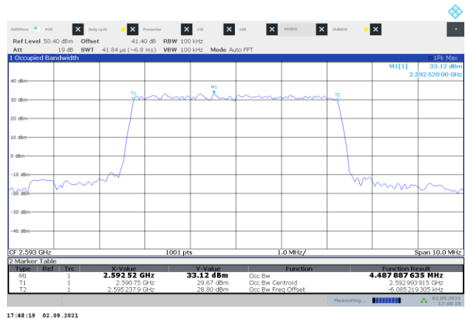
Figure 8.4-2: 99% OBW sample plot for 5 MHz channel
