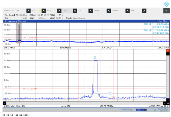
Figure 8.3-56: Conducted spurious emissions at Ant 2 64QAM 20 MHz mid channel
