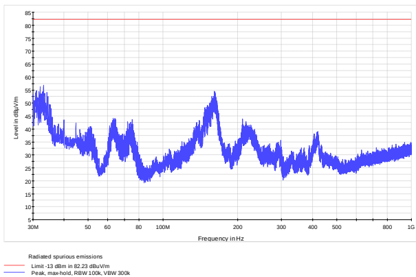
Figure 8.3-63 Cabinet spurious radiations 30–1000 MHz for top channel
