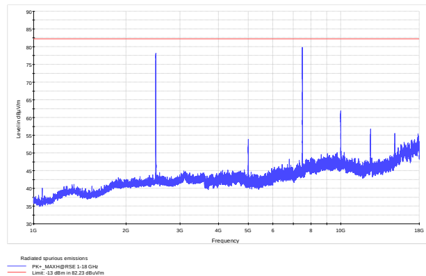
Figure 8.3-64: Cabinet spurious radiations 1–18 GHz for low channel
