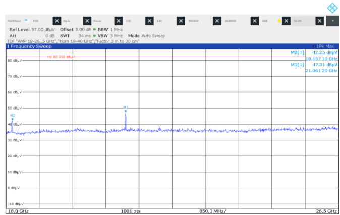
Figure 8.3-68 Cabinet spurious radiations 18–26.5 GHz for mid channel
