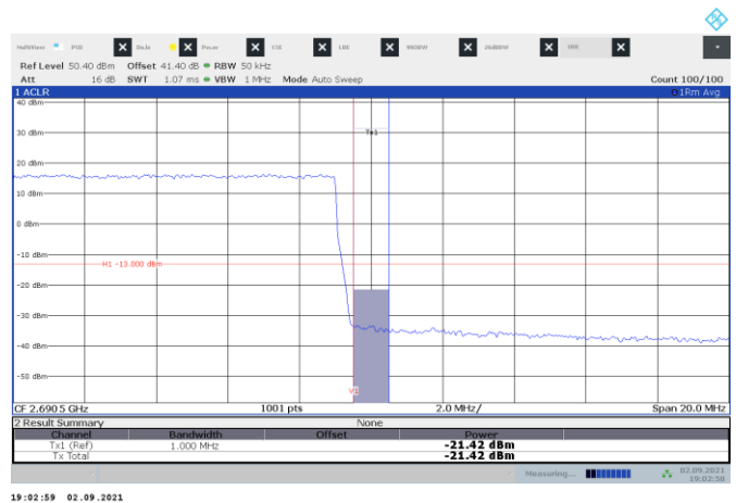
Figure 8.3-12: Band edge measurement for Ant 2 QPSK 10 MHz top channel
