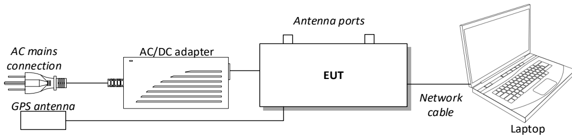
Figure 5.6-1: Setup diagram
