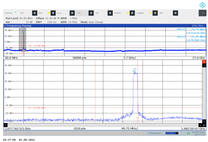
Figure 8.3-60: Conducted spurious emissions at Ant 2 64QAM 20 MHz top channel
