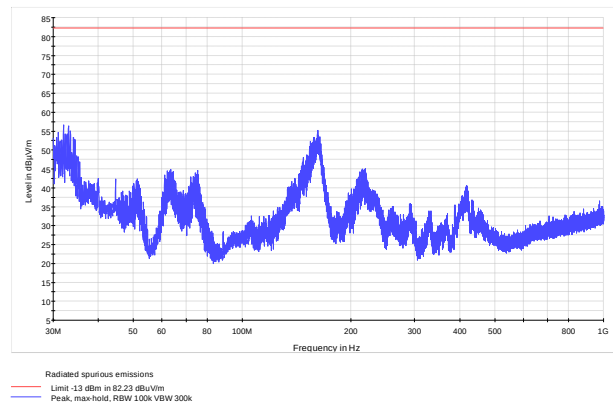
Figure 8.3-62: Cabinet spurious radiations 30–1000 MHz for mid channel
