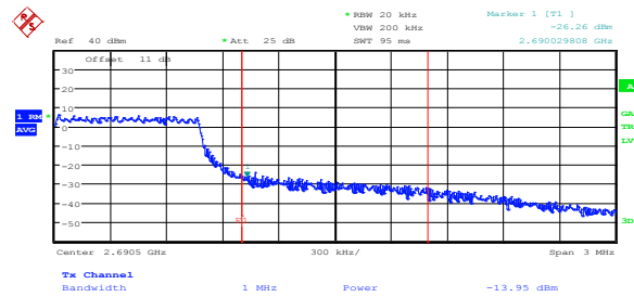
Figure 8.2-56: Conducted upper band edge emissions at antenna port 2, 2.5 MHz BW, 256-QAM
