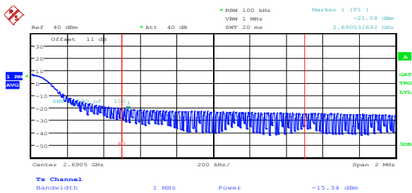
Figure 8.2-57: Conducted upper band edge emissions at antenna port 1, 5 MHz BW, BPSK
