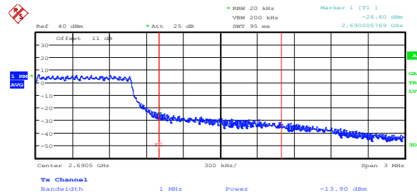
Figure 8.2-54: Conducted upper band edge emissions at antenna port 2, 2.5 MHz BW, BPSK
