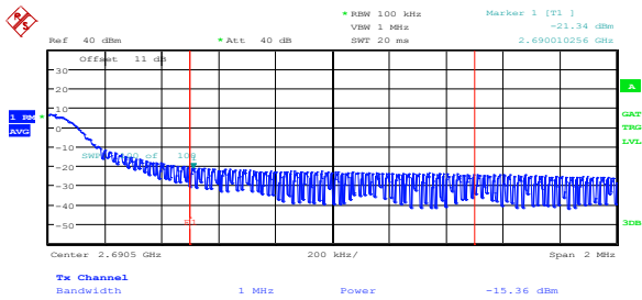
Figure 8.2-59: Conducted upper band edge emissions at antenna port 1, 5 MHz BW, 256-QAM
