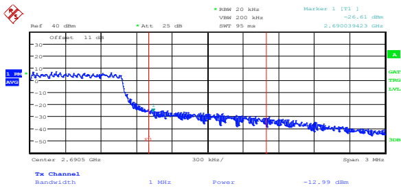
Figure 8.2-55: Conducted upper band edge emissions at antenna port 1, 2.5 MHz BW, 256-QAM
