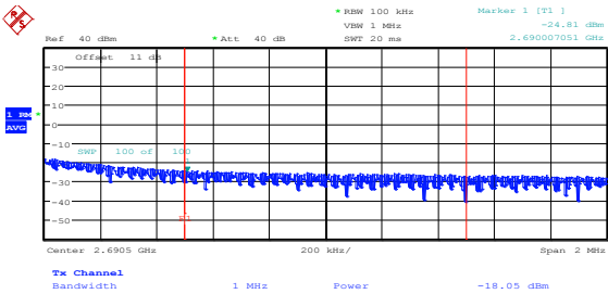
Figure 8.2-63: Conducted upper band edge emissions at antenna port 1, 10 MHz BW, 256-QAM
