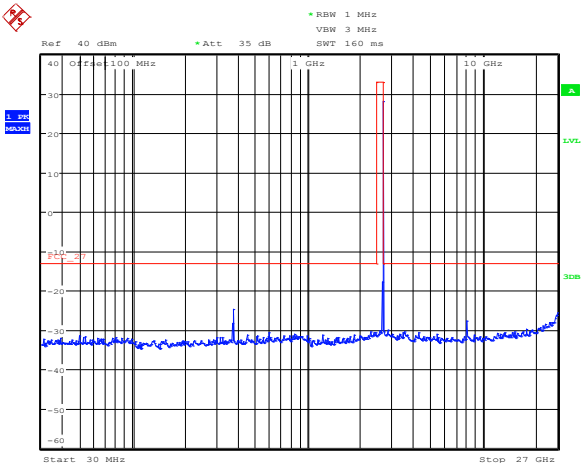
Figure 8.2-3: Conducted spurious emissions at antenna port 1, low channel, 1.25 MHz BW, 256-QAM
