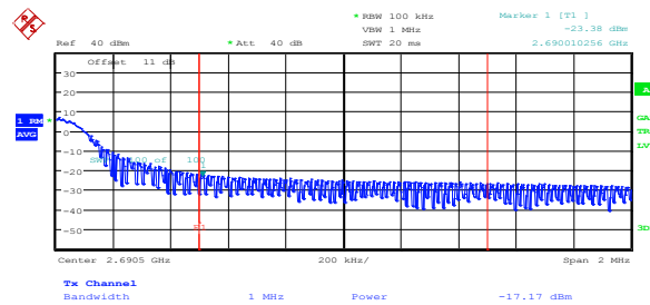
Figure 8.2-58: Conducted upper band edge emissions at antenna port 2, 5 MHz BW, BPSK
