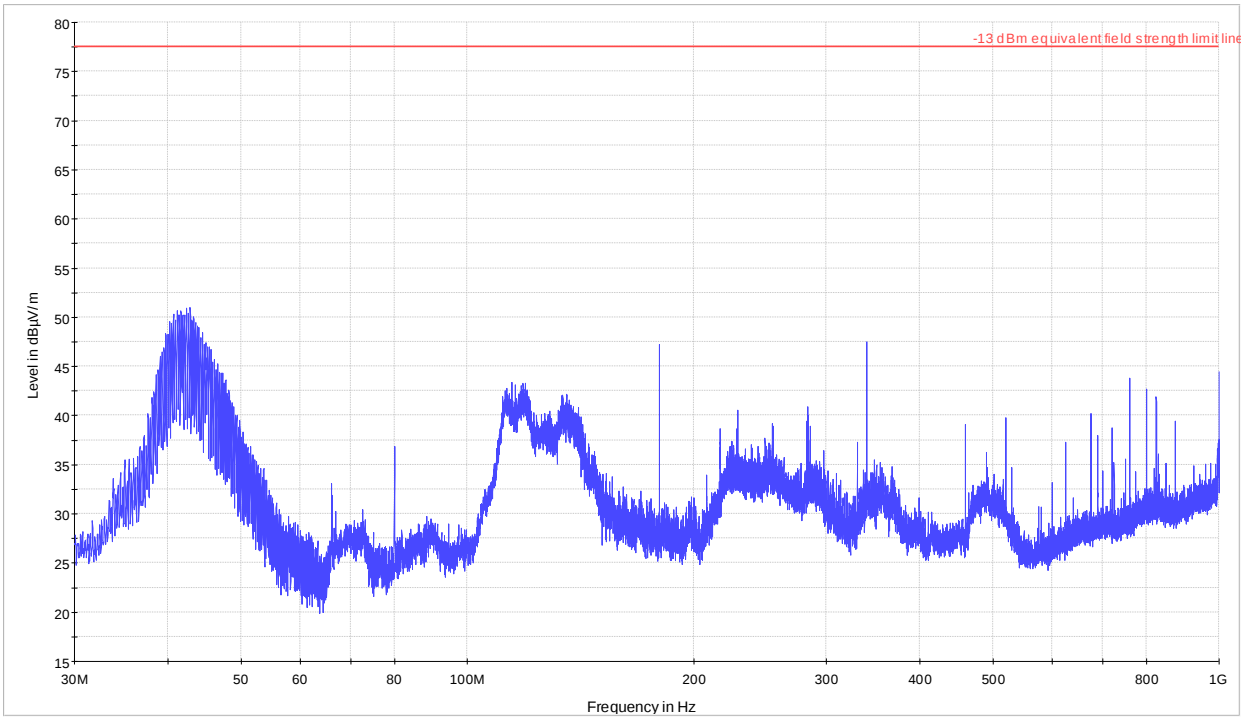
Figure 8.2-65: Cabinet radiation below 1 GHz, sample plot
