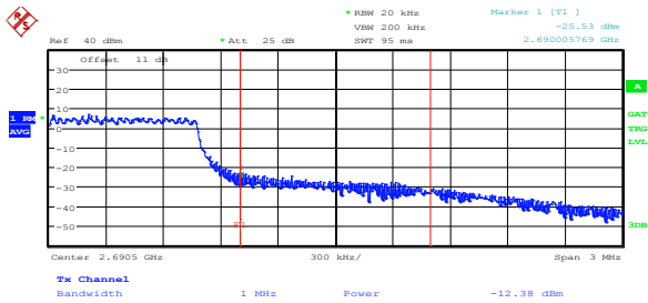
Figure 8.2-53: Conducted upper band edge emissions at antenna port 1, 2.5 MHz BW, BPSK
