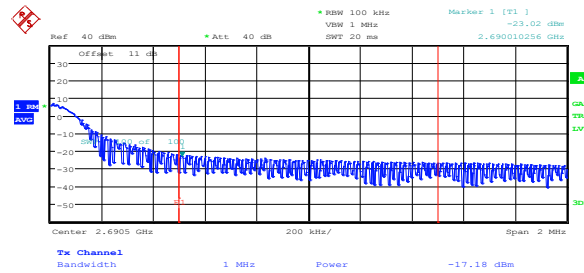
Figure 8.2-60: Conducted upper band edge emissions at antenna port 2, 5 MHz BW, 256-QAM
