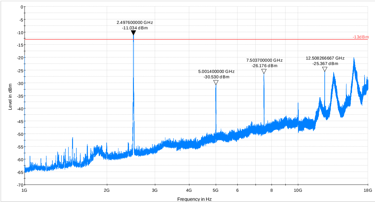
Figure 8.2-66: Cabinet radiation above 1 GHz, sample plot
