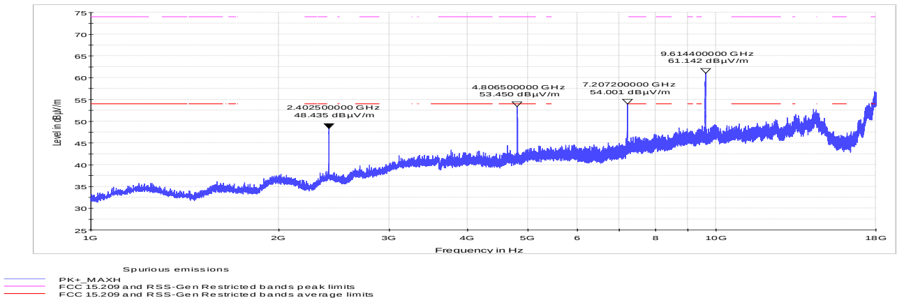
Figure 8.4-4: Radiated spurious emissions for 5 MHz, low channel
