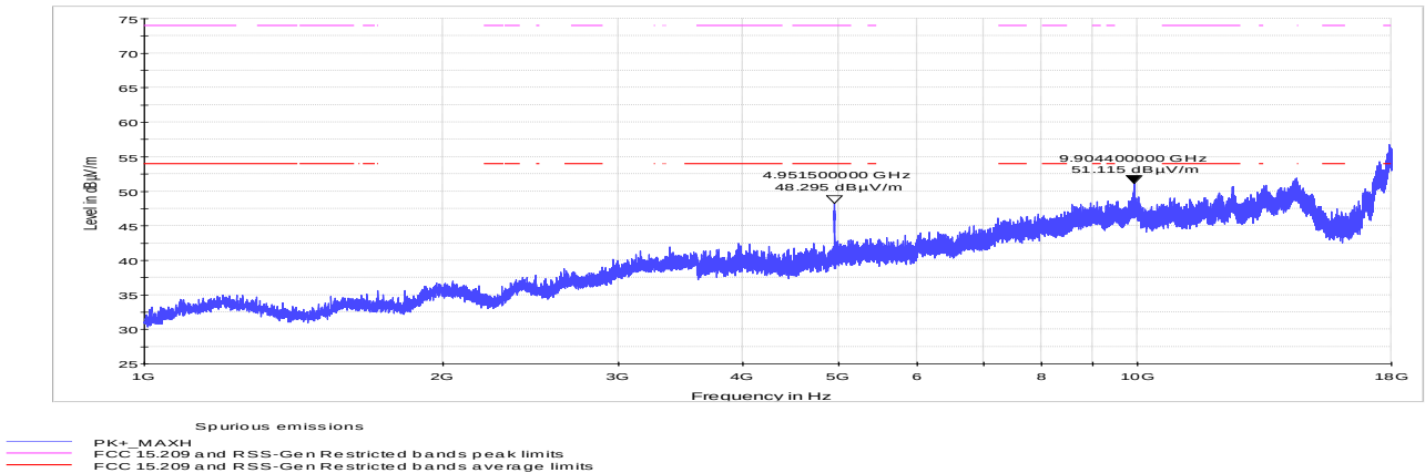
Figure 8.4-6: Radiated spurious emissions for 5 MHz, high channel
