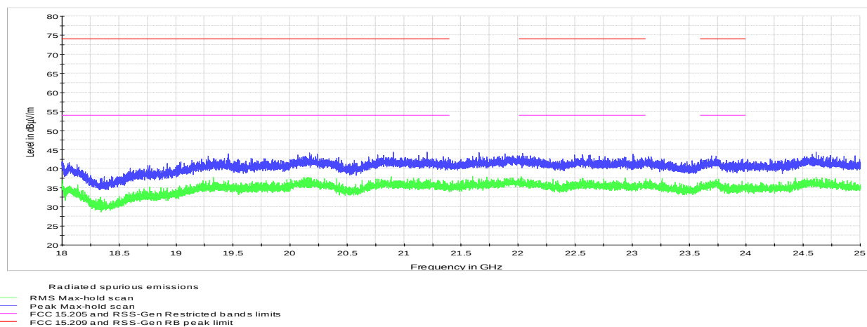
Figure 8.4-15: Radiated spurious emissions for 5 MHz, high channel
