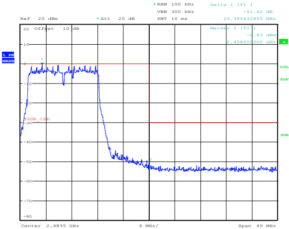
Figure 8.4-112: Conducted spurious emissions outside restricted bands at the upper band edge, 5 MHz high channel, Ant 1
