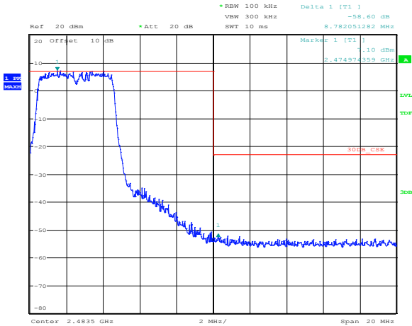
Figure 8.4-113: Conducted spurious emissions outside restricted bands at the upper band edge, 10 MHz high channel, Ant 1
