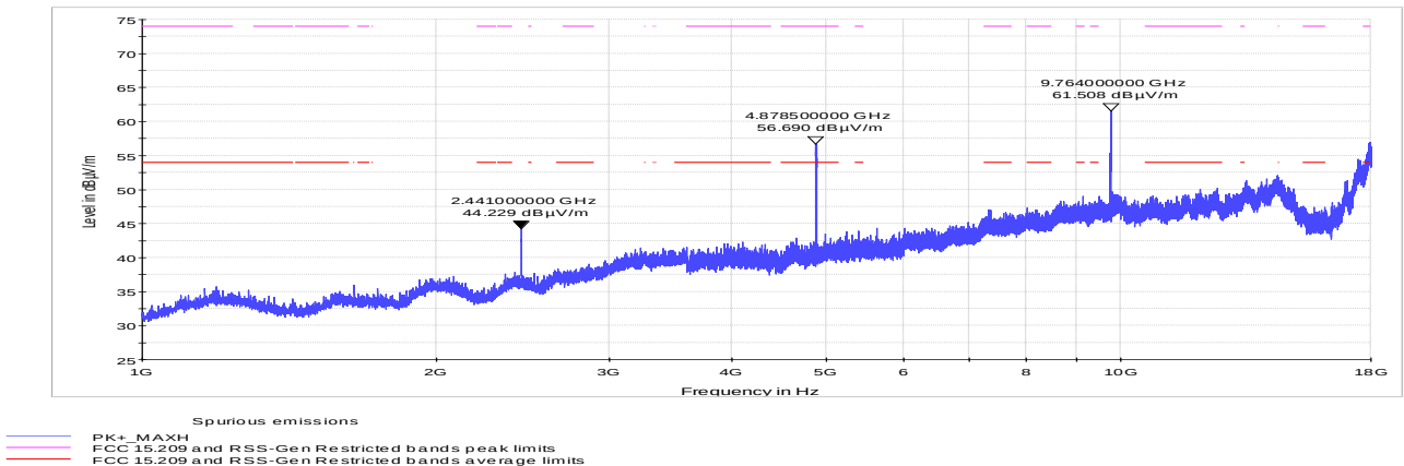
Figure 8.4-5: Radiated spurious emissions for 5 MHz, mid channel
