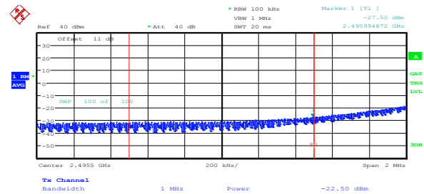
Figure 8.2-48: Conducted lower band edge emissions at antenna port 2, 10 MHz BW, 256-QAM
