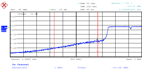
Figure 8.2-35: Conducted lower band edge emissions at antenna port 1, 1.25 MHz BW, 256-QAM
