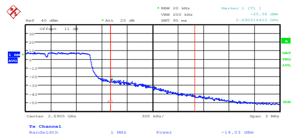
Figure 8.2-52: Conducted upper band edge emissions at antenna port 2, 1.25 MHz BW, 256-QAM
