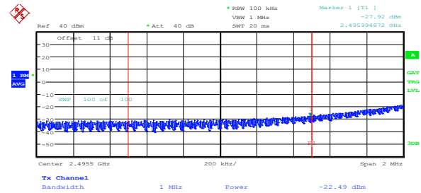
Figure 8.2-46: Conducted lower band edge emissions at antenna port 2, 10 MHz BW, BPSK
