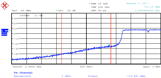
Figure 8.2-33: Conducted lower band edge emissions at antenna port 1, 1.25 MHz BW, BPSK
