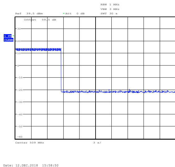
Figure 8.3-5: Unsuccessful registration with restricted coordinates. Spectrum plot shows that prior to the unsuccessful registration the EUT was transmitting and the transmission stopped right after the EUT detected missing information in the registration form.
