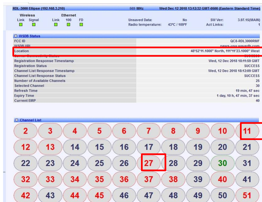
Figure 8.19-8: Received channel list for coordinates set in scenario (a) and (b). LPT channel 27 and TV receive site channel 11 at location coordinates 48.87N, 111.19W
