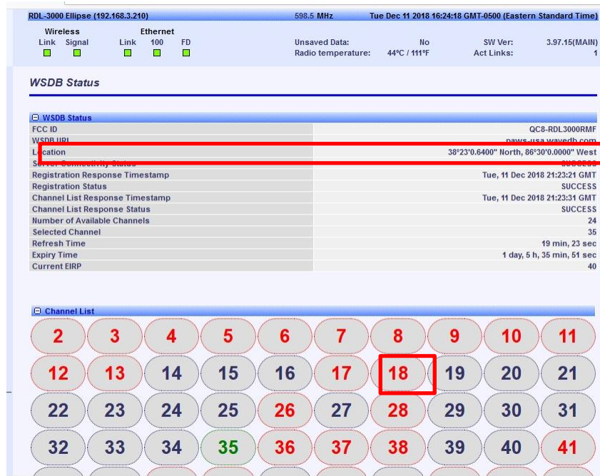
Figure 8.19-1: Received channel list for coordinates set in scenarios (a) and (b). DCA channel 18 at location coordinates 38.4N, 86.5W
