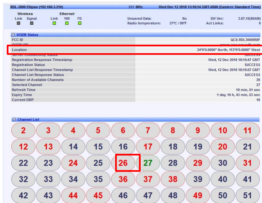
Figure 8.19-9: Received channel list for coordinates set in scenario (a) and (b). MVPD channel 26 at location coordinates 34.0N, 113.0W
