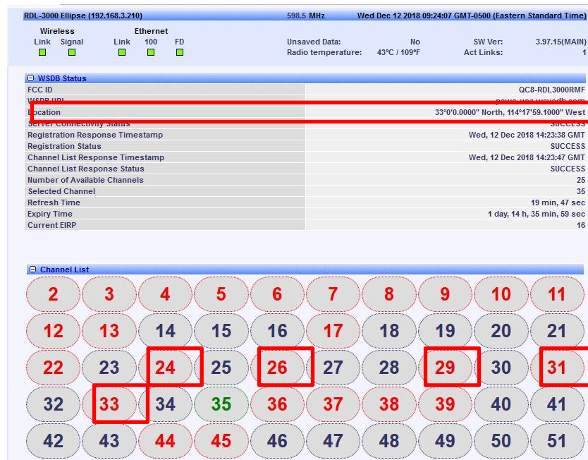
Figure 8.19-5: Received channel list for coordinates set in scenario (a) and (b). LPX channels 24, 26, 29, 31, and 33 at location coordinate 33N, 114.3W
