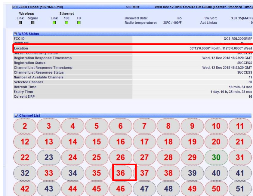
Figure 8.19-10: Received channel list for coordinates set in scenario (c). Permanent BAS link channel 36 at location coordinates 33.2N, 112.0W
