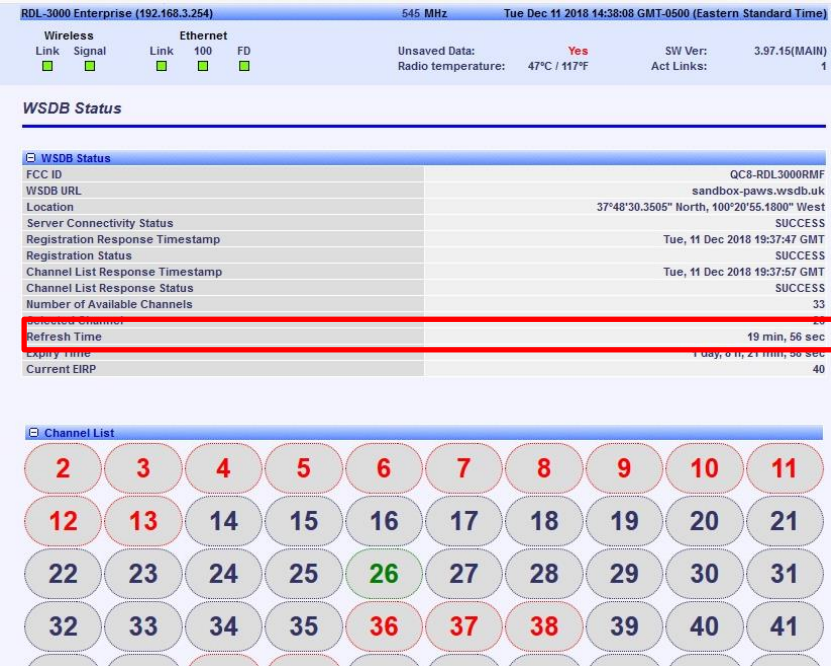
Figure 8.2-2: Refresh time instead of 48-hour push notification wait of subscriber device
