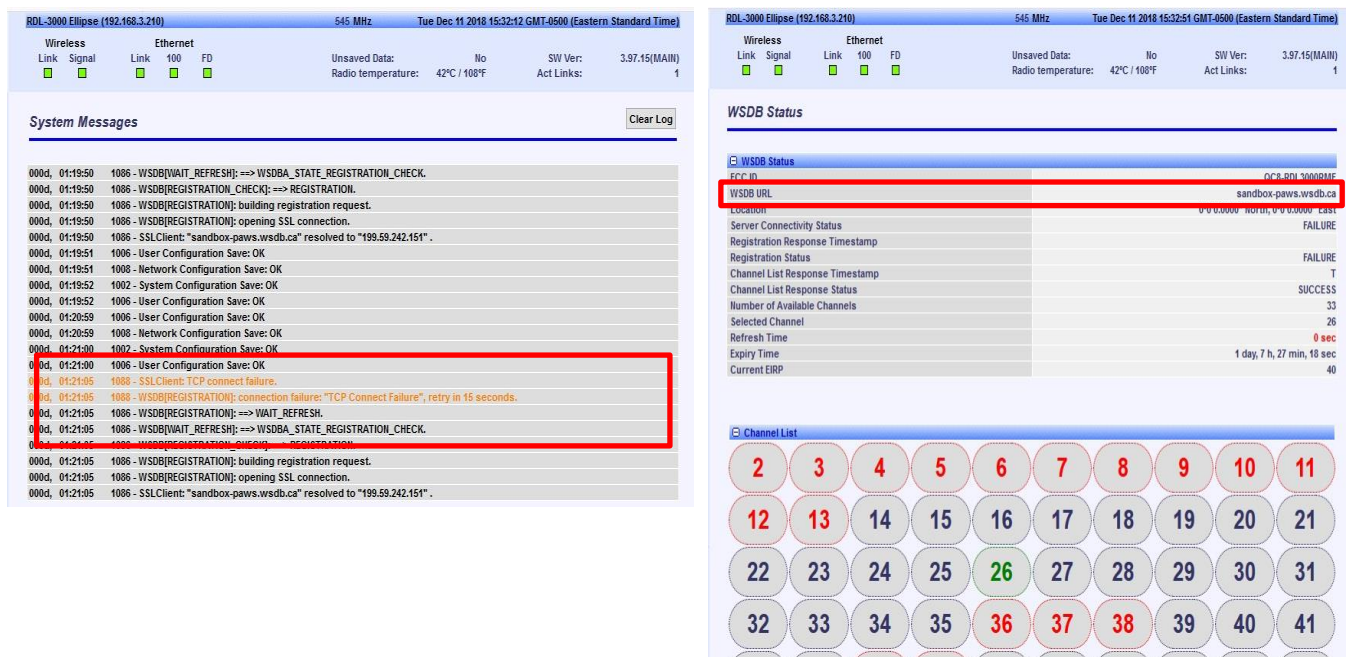
Figure 8.17-1: Data log of unsuccessful registration due to wrong database URL of Base station device
