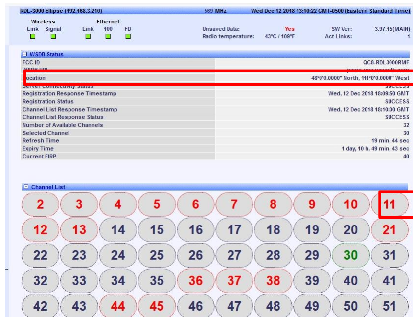
Figure 8.19-7: Received channel list for coordinates set in scenario (a) and (b). LPD channel 11 at location coordinates 48.0N, 111.0W
