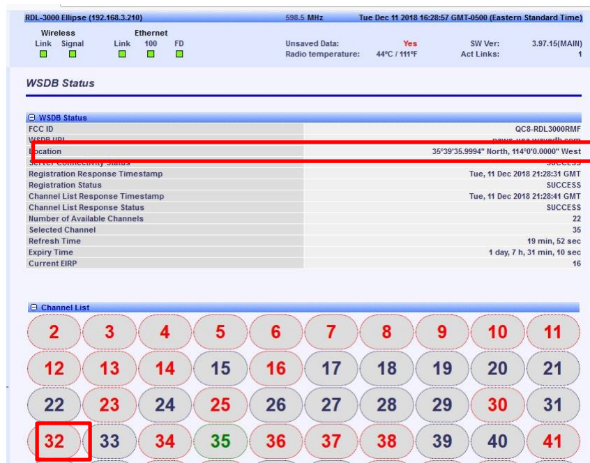
Figure 8.19-3: Received channel list for coordinates set in scenarios (a) and (b). DTS channel 32 at location coordinates 35.66N, 114.0W
