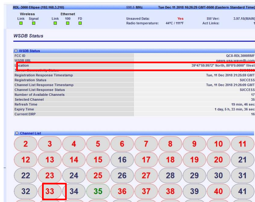
Figure 8.19-2: Received channel list for coordinates set in scenarios (a) and (b). DRT channel 33 at location coordinates 39.8N, 80.0W
