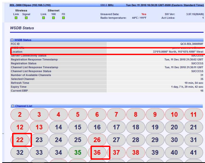
Figure 8.19-4: Received channel list for coordinates set in scenarios (a) and (b). DTV channels 22 and 36 at location coordinate 33.0N, 115.3W
