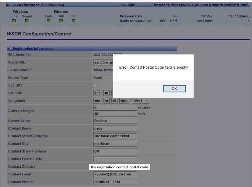
Figure 8.9-2: Data log of unsuccessful registration with missing contact zip (postal) code of Subscriber device
