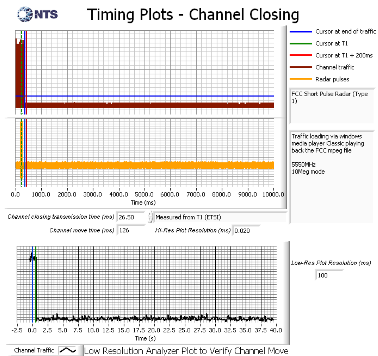
Figure 6 Channel Closing Time and Channel Move Time – Type 1 - 10MHz – 40 second plot
